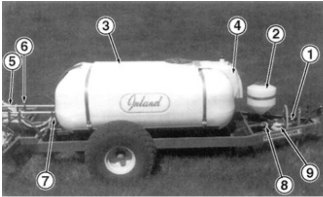
FIGURE 1. Inland Model Terminator I Auto-Fold Field Sprayer: (1) Hydraulic Motor and Pump, (2) Easy-Fill Chemical Tank, (3) Spray Tank, (4) Clean Water Tank, (5) Spray Boom, (6) Nozzle Body Assembly, (7) Solenoid and Regulator Valves, (8) Agitator Valve and (9) Strainer.
