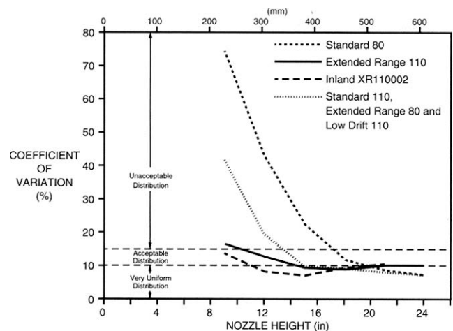
FIGURE 6. Spray pattern uniformity for flat fan extended, standard and low drift flat fan stainless steel nozzles.
