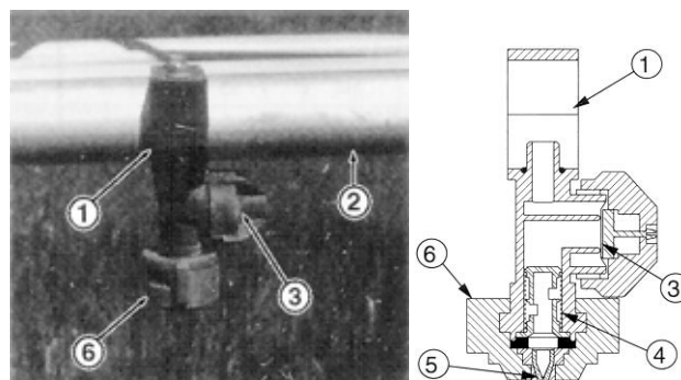
FIGURE 8. Spraying Systems Diaphragm and Nozzle Body Assembly: (1) Split-Eyelet Clamp, (2) Spray Boom, (3) Diaphragm Check Valve, (4) Strainer, (5) Nozzle Tip and (6) Quick-Disconnect and Self-Aligning Nozzle Cap.
