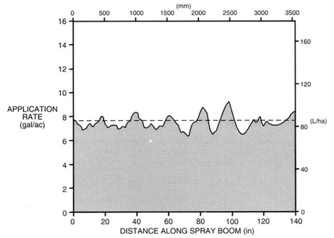
FIGURE 4. Distribution pattern along the boom at 44 psi (300 kPa) with Spraying Systems extended range Tee Jet XR11002VS stainless steel nozzle tips, at a 12 in (300 mm) nozzle height and 7 mph (11 km/h).
