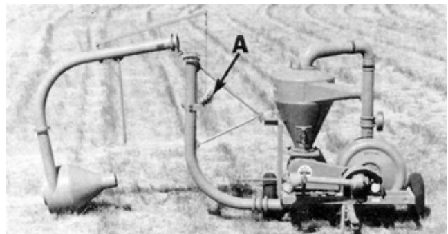
FIGURE 3. Cyclone Resting on Ground for Convenient Attaching: (A) Winch.
