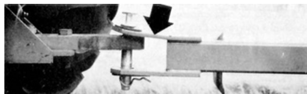
FIGURE 15. Bent Hitch Clevis.
