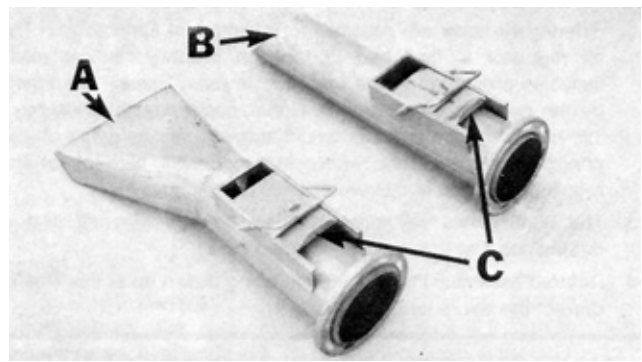
FIGURE 6. Intake Nozzles: (A) Flat Nozzle, (B) Round Nozzle, (C) Adjustable Slide.
