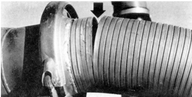
FIGURE 18. Cracked Flexible Piping at Separator Cyclone Inlet.
