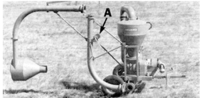
FIGURE 8. Transport Position: (A) Winch.
