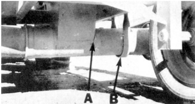
FIGURE 17. Cracked Discharge Tube: (A) Crack, (B) Supporting Brace.
