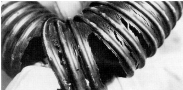
FIGURE 14. Failure of Polyurethane Hose due to Weathering.
