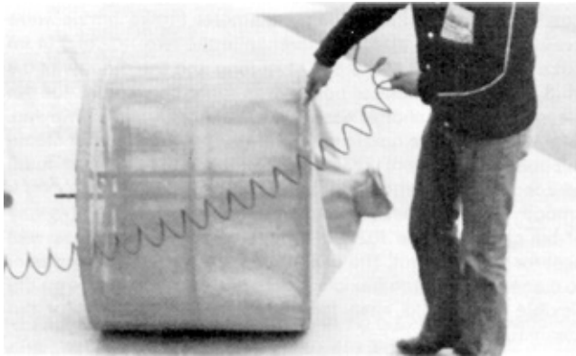
FIGURE 5. Filter Bag.
