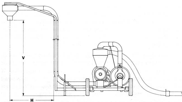
FIGURE 2. Standard Discharge Assembly ( V = 3.9 m, H = 1.7 m).
