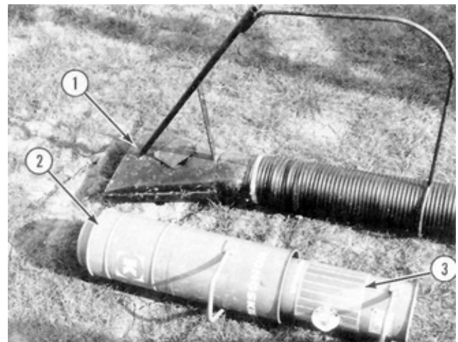
FIGURE 3. Intake Nozzles: (1) Flat Nozzle, (2) Round Nozzle, (3) Adjustable Sleeve.
