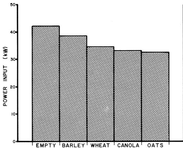
FIGURE 16. Power Requirements at Maximum Conveying Rates.
