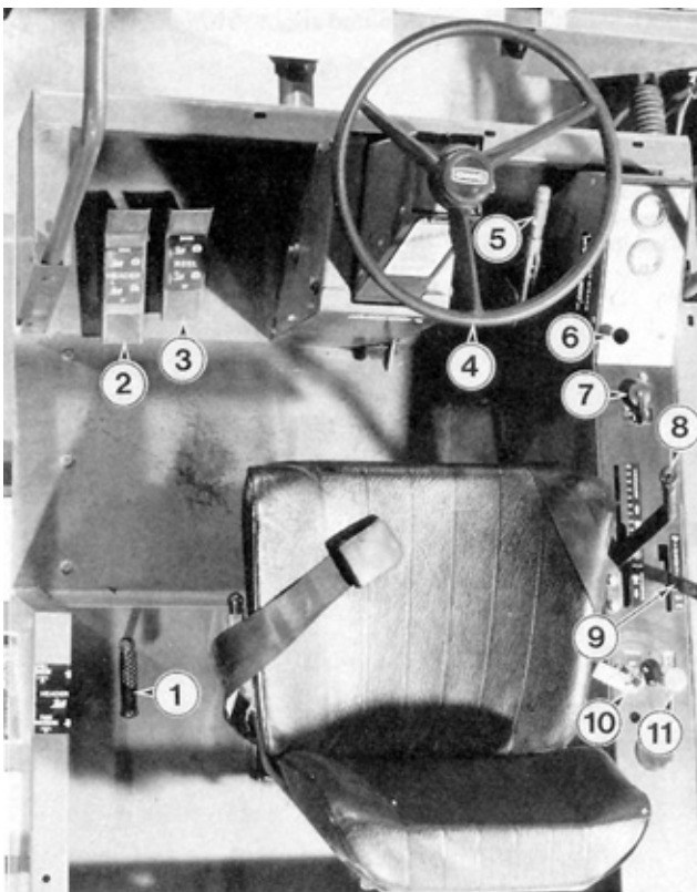
FIGURE 2. Operator Station. (1) Header drive control (2) Header height control pedal (3) Reel height control pedal (4) Steering wheel (5) Parking brake (6) Warning lights switch (7) Turn indicator switch (8) Travel speed control lever (9) Throttle (10) Ignition switch (11) Choke.
