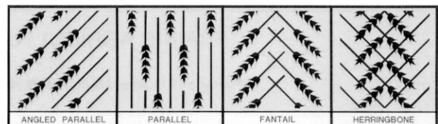
FIGURE 1. Windrow Types.
