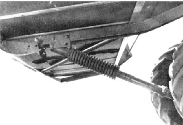
FIGURE 15. Header Float Springs.
