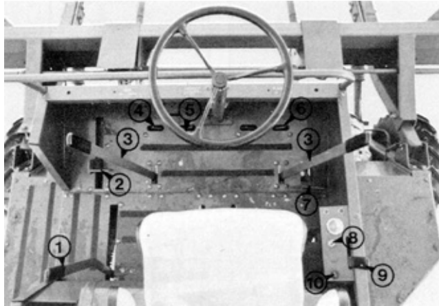
FIGURE 1. Operator's Platform.
