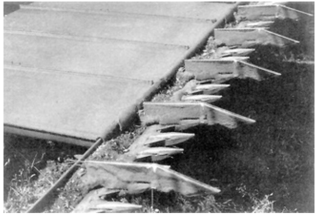
FIGURE 9. Rigid Type Vine Lifter Attachments.
