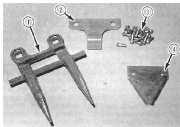
FIGURE 1. MacDon Conventional: 1) Guard, 2) Hold-down Clip, 3) Rivets, 4) Knife Section (typically pre-assembled on bar).
