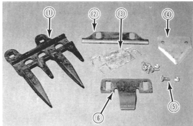
FIGURE 7. Crary 4 in 1: 1) Guard, 2) Wear Plate, 3) Shims, 4) knife Section, 5) Bolts, 6) Hold-down Clip.
