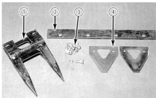
FIGURE 3. Schumacher Easy-Cut: 1) Guard, 2) Spacer Bar, 3) Bolts, 4) Knife Sections.
