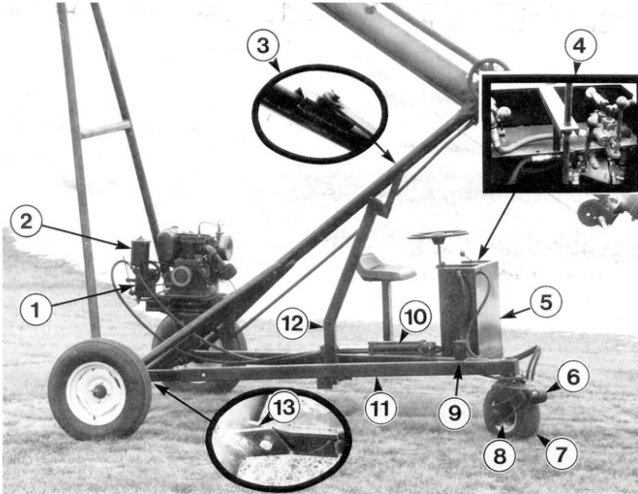
FIGURE 1. (1) Hydraulic pump, (2) Hydraulic oil reservoir, (3) Lift bracket, (4) Hydraulic controls, (5) Operator platform, (6) Hydraulic motor, (7) Drive wheel, (8) Drive chain, (9) Transport bracket, (10) Hydraulic cylinder, (11) Telescopic frame, (12) Lift arms, (13) Mounting brackets.
