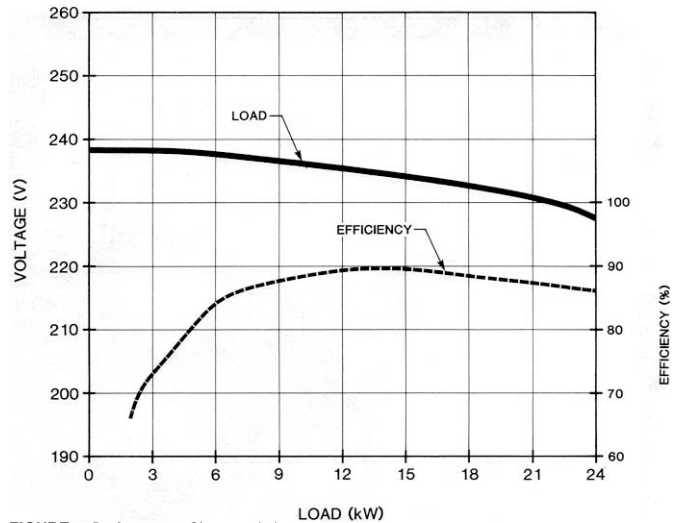
FIGURE 2. Performance Characteristics.
