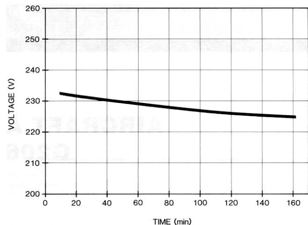
FIGURE 3. Endurance Test.
