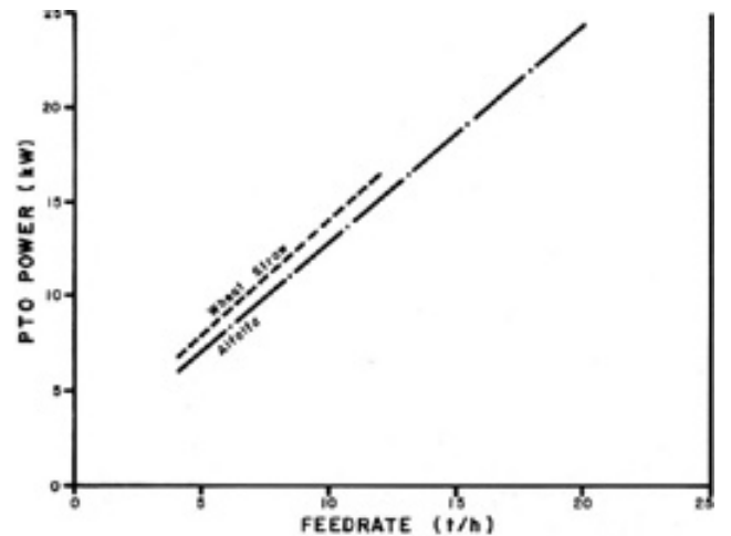
FIGURE 6. Average Power Take-off Requirements when Baling Alfalfa and Straw.
