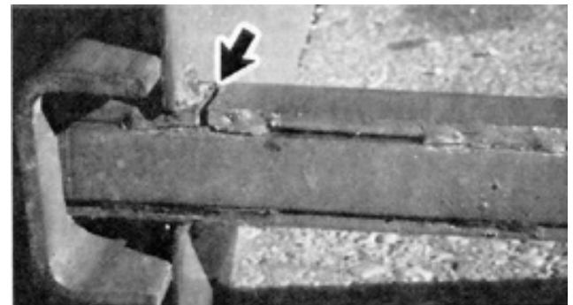
FIGURE 12. Failure of Bale Chute Frame Welds.
