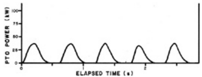
FIGURE 5. Instantaneous Power Take-off Requirements when Baling Alfalfa at 10 t/h Feedrate.
