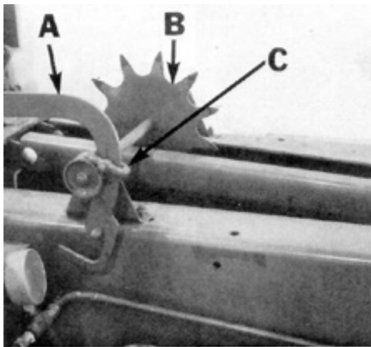
FIGURE 4. Bale Length Adjustment: (A) Metering Arm, (B) Metering Wheel, (C) Adjustable Stop.
