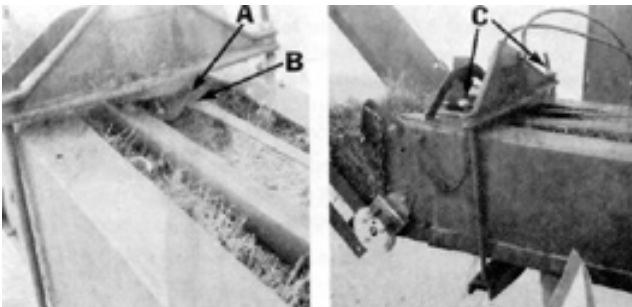
FIGURE 9. Bent Hydraulic Ram Linkages: (A) Cross Piece, (B) Tension Rail, (C) Tension Rod.
