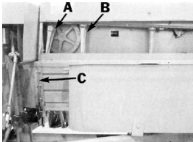
FIGURE 7. Feeder Adjustments: (A) Left Feed Tines, (B) Centre Feed Tines, (C) Feeder Back.
