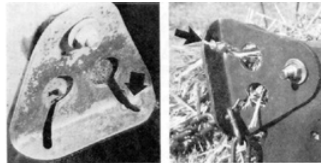
FIGURE 11. Deformed and Cracked Bale Chute Brackets.
