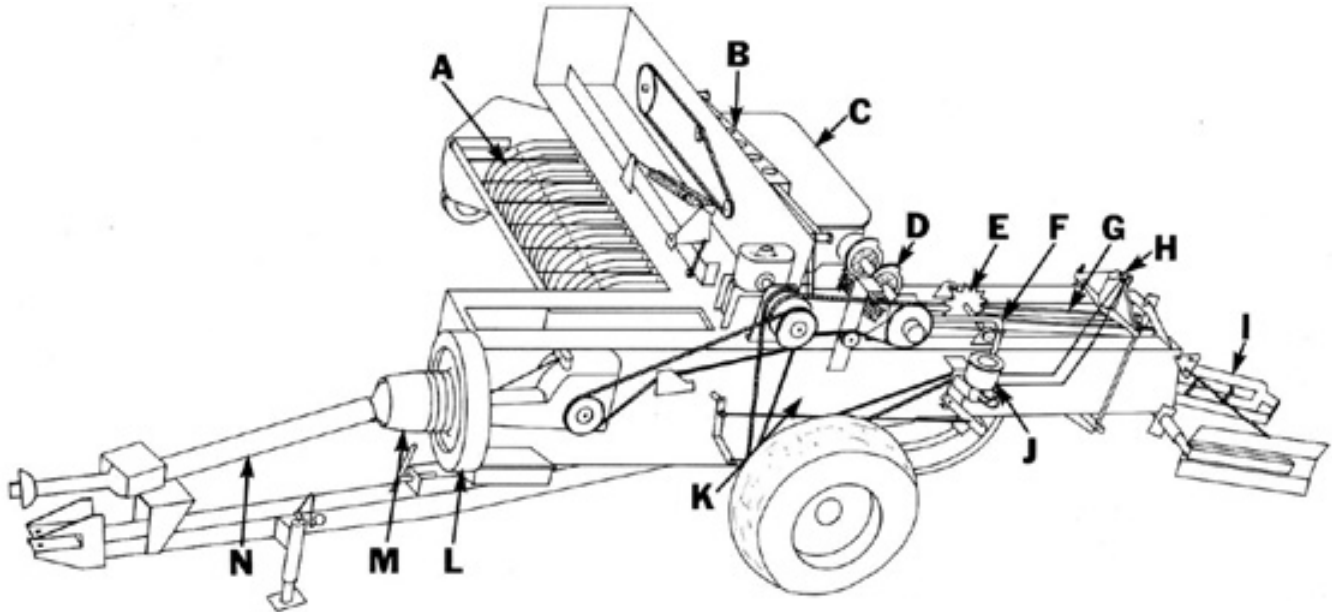
FIGURE 1. New Holland 320 Baler: (A) Pickup, (B) Tine Bar Feeder, (C) Twine Box, (D) Knotter, (E) Metering Wheel, (F) Metering Arm, (G) Pressure Bar, (H) Hydraulic Bale Density Ram, (I) Bale Chute, (J) Hydraulic Bale Density Pump and Control (K) Bale Chamber, (L) Flywheel, (M) Slip Clutch, (N) Power Shaft.
