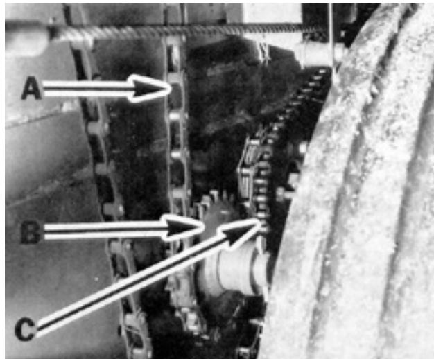
FIGURE 8. Interference Between the Pickup Drive Sprocket and Optional Hydraulic Bale Density Pump Drive Chains: (A) Pickup Drive Chain, (B) Pickup Drive Sprocket, (C) Pump Chain Drive.
