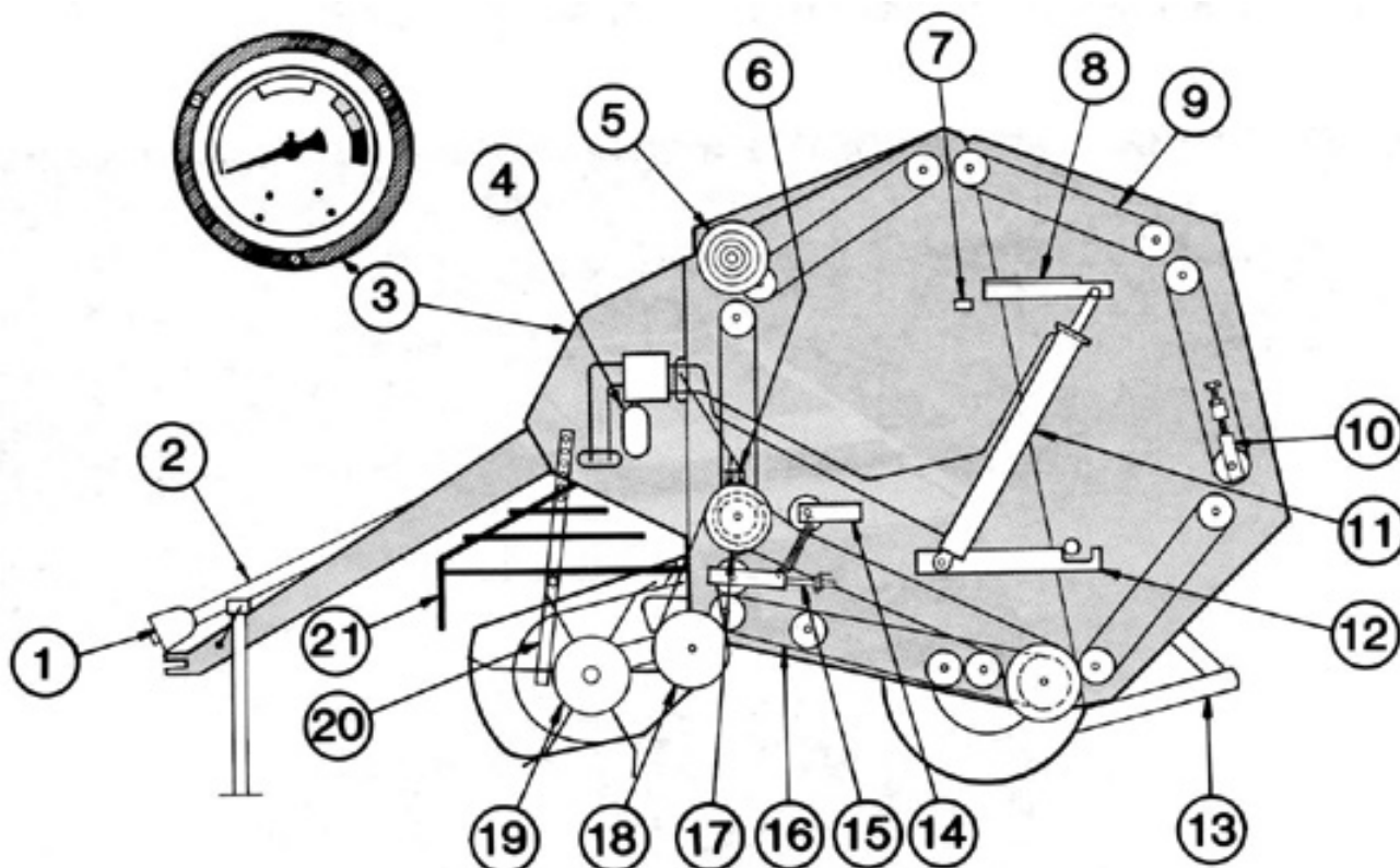
FIGURE 1. Vicon RP 1510/CI 560 Round Baler: (1) Constant Velocity PTO, (2) Drive Shaft, (3) Density Gauge, (4) Accumulator, (5) Twine Driving Wheel, (6) Automatic Chain Oiler Brushes, (7) Bale Counter, (8) Gate Lock, (9) Upper Forming Belts, (10) Adjusting Block, (11) Gate Cylinder, (12) Gate Latch, (13) Bale Kicker, (14) Chain Idler, (15) Belt Tensioner, (16) Platform Belts, (17) Main Drive Roller, (18) Pickup Pivot Shaft, (19) Pickup, (20) Transport Arm, (21) Pickup Guard.
