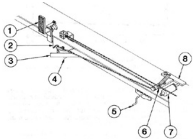
FIGURE 5. Twine Tying Mechanism: (1) Reflector, (2) Twine Guide, (3) Twine Holder, (4) Twine Knife, (5) Twine Adjustment Rod, (6) Twine Arm, (7) Solenoid, (8) Trip Lever.
