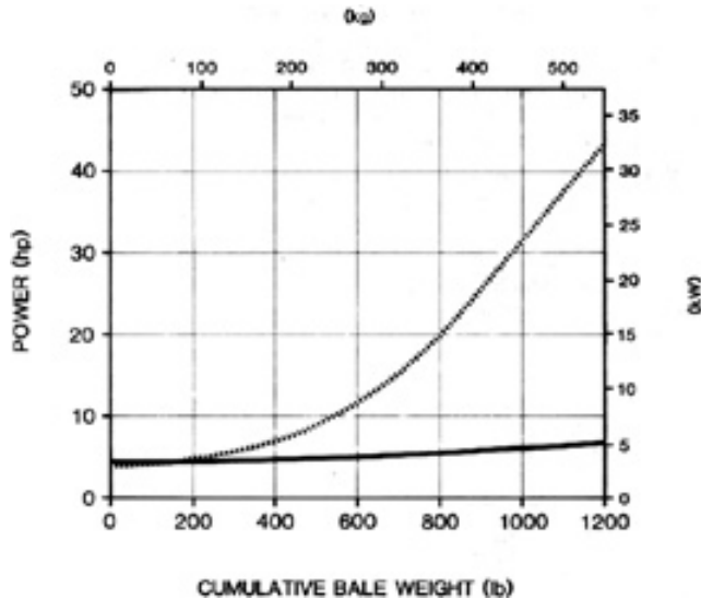
FIGURE 7. Power Consumption During Bale Formation in Alfalfa Bromegrass.
