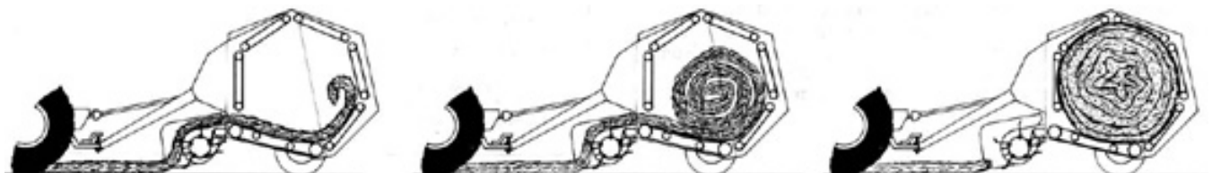
FIGURE 4. Stages of Bale Formation.
