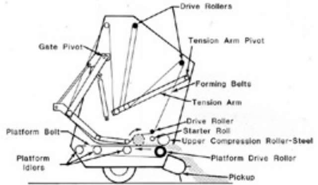
Figure 1. Schematic View of John Deere 500 Round Baler.
