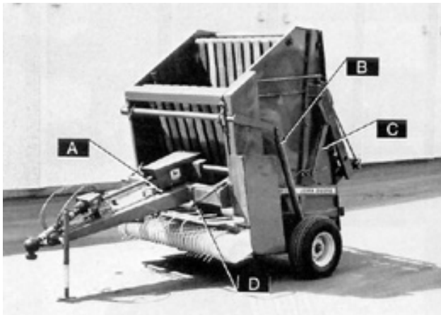
Figure 2. Front View of John Deere 500 Round Baler. Identification of Components: (A) Twine Cylinder, (B) Tension Spring, (C) Gate Cylinder, (D) Pickup Transport Lever.
