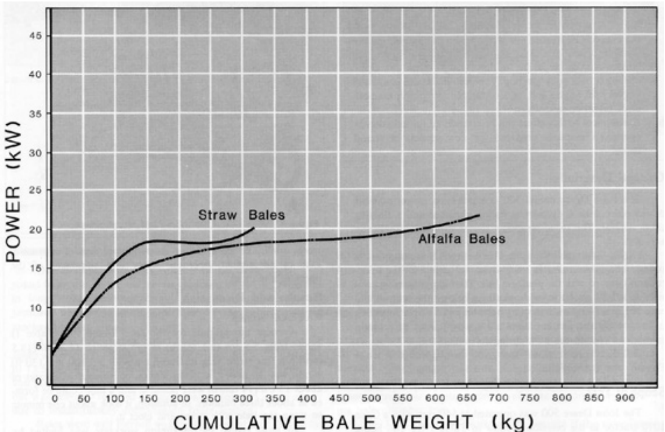
Figure 6. Power Consumption of the John Deere 500 During Bale Formation.
