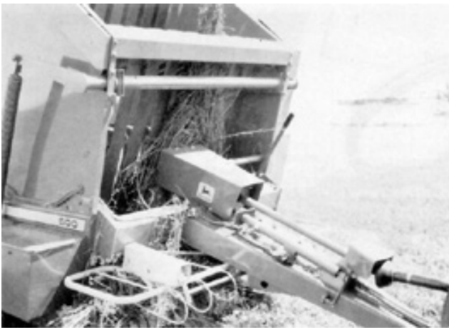
Figure 9. Plugging in Sweet Clover Before Compression Roll Modification.
