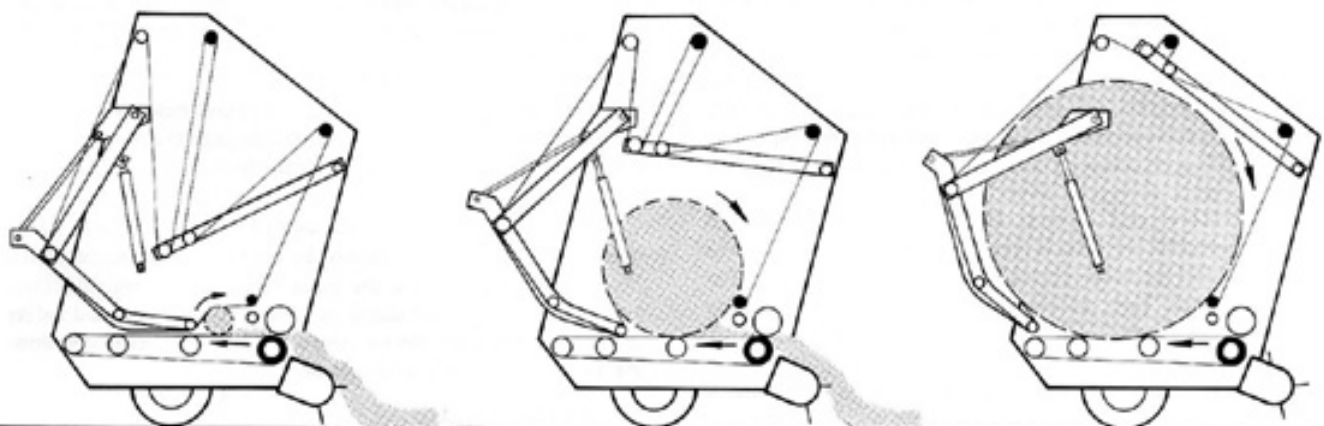
Figure 7. Stages of Bale Formation: (Left) Bale Core, (Centre) Half-Completed Bale, (Right) Completed Bale.
