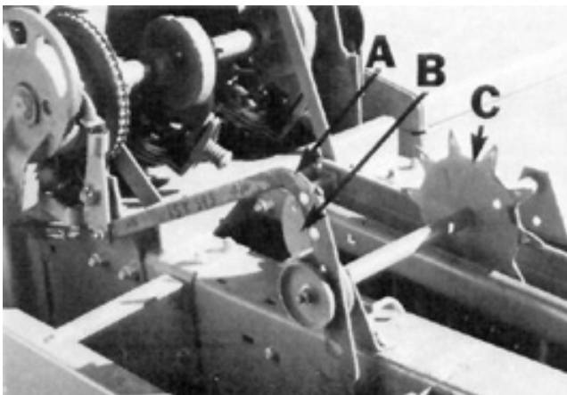
FIGURE 3. Bale Length Adjustment: (A) Metering Arm, (B) Adjustable Stop, (C) Metering Wheel.
