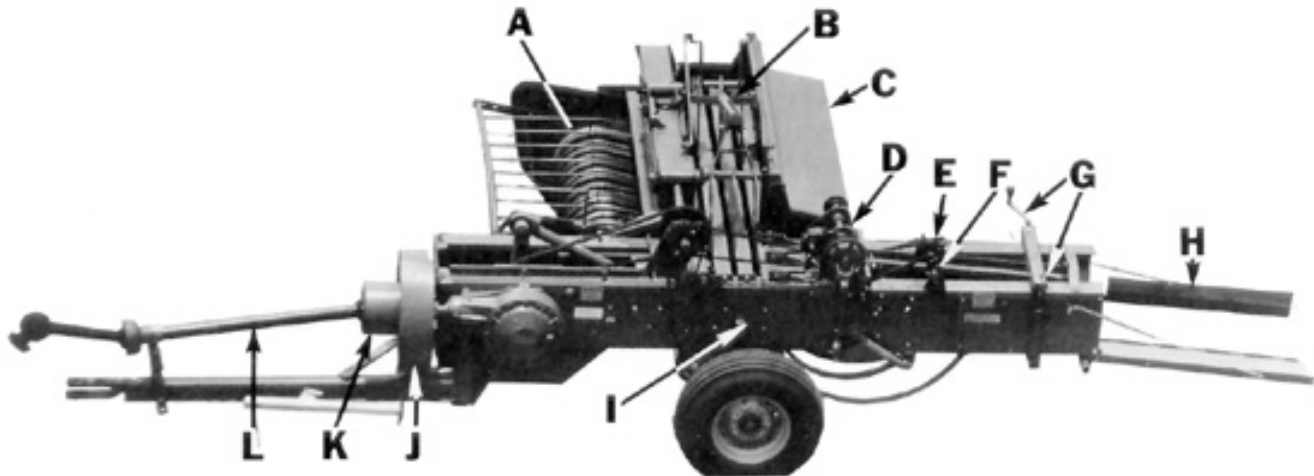
FIGURE 1. Massey Ferguson 124 Baler: (A) Pickup, (B) Packer Fork, (C) Twine Box, (D) Knotters, (E) Metering Wheel, (F) Metering Arm, (G) Bale Density Adjustment, (H) Quarter Turn Bale Chute, (I) Bale Chamber, (J) Flywheel, (K) Slip Clutch, (L) Power Shaft.
