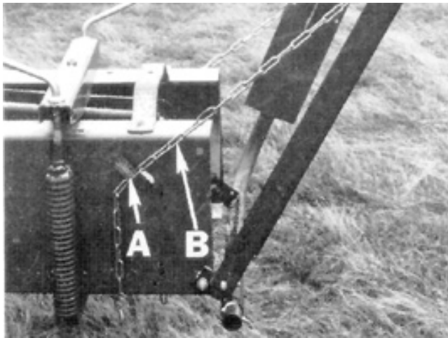
FIGURE 6. Bale Chute in Transport Position: (A) Hook, (B) Link.
