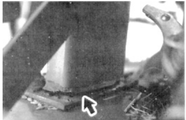
FIGURE 9. Broken Knottter Mounting Frame.
