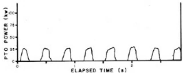
FIGURE 4. Instantaneous Power Take-off Requirements when Baling Alfalfa at 8 t/h Feedrate.
