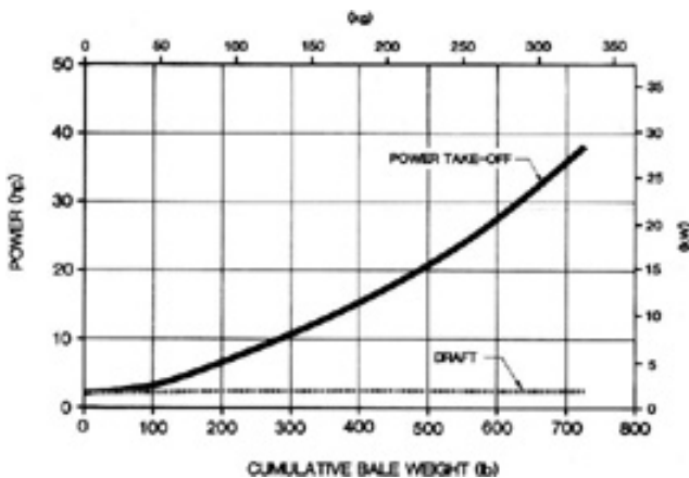
FIGURE 4. Power Consumption During Bale Formation in Alfalfa-Bromegrass.
