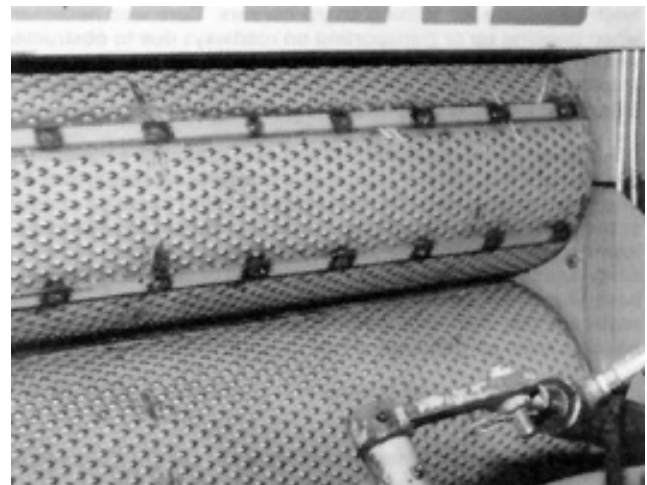
FIGURE 6. Bars Mounted to Alternate Rollers at Front.
