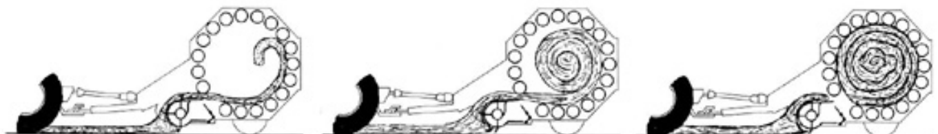
FIGURE 5. Stages of Bale Formation: (Left) Starting Bale, (Centre) Partially Completed Bale, (Right) Completed Bale.
