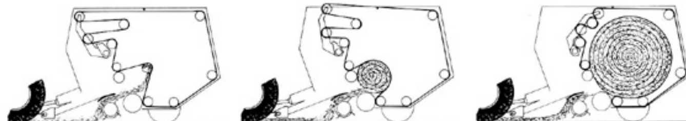
FIGURE 4. Stages of Bale Formation: (Left) Starting Bale, (Centre) Partially Completed Bale, (Right) Completed Bale.
