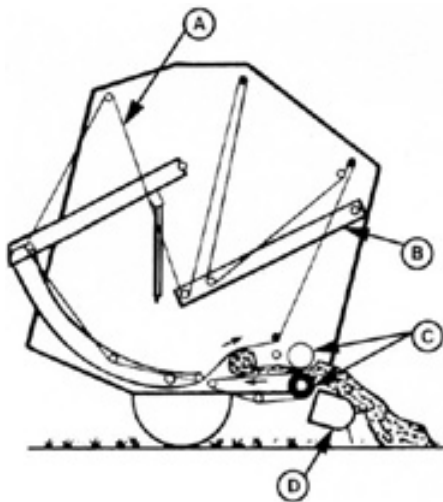
FIGURE 1. John Deere 510 Round Baler: (A) Bale Forming Belts, (B) Tensioning Arm, (C) Compression Rollers, (D) Pickup.
