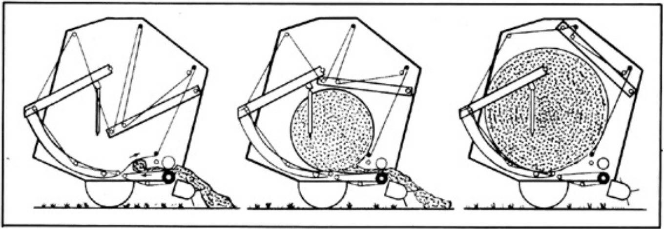
FIGURE 5. Stages of Bale Formation: (Left) Bale Core, (Centre) Half-Completed Bale, (Right) Completed Bale.
