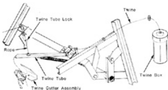
FIGURE 6. Twine Wrapping Mechanism.
