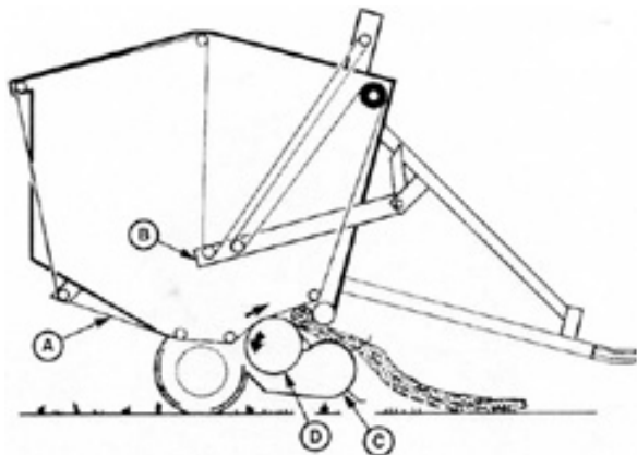
FIGURE 1. Vermeer 605E (A) Bale Forming Belts, (B) Tension Arm, (C) Pickup, (D) Platform Roller.
