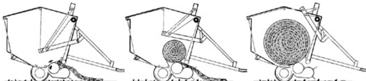
FIGURE 5. Stages of Bale Formation: (Left) Bale Core, (Centre) Half-Completed Bale, (Right) Completed Bale.
