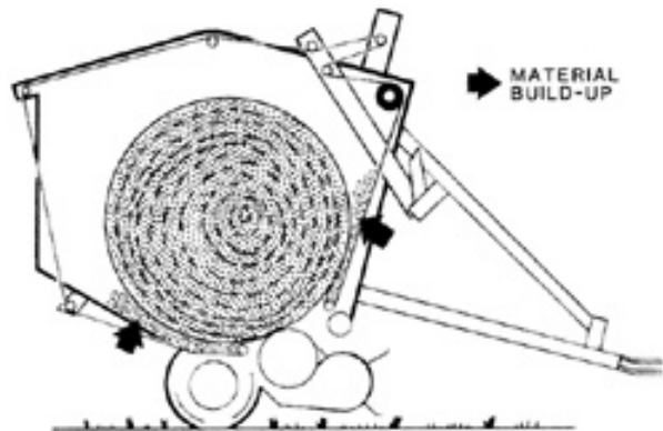
FIGURE 8. Hay Buildup Between Belts.
