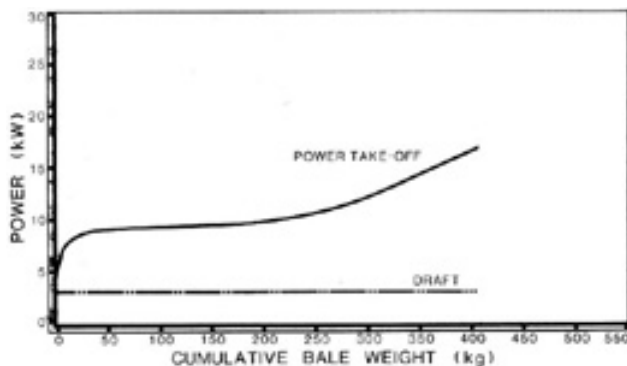
FIGURE 4. Power Consumption During Bale Formation in Alfalfa.
