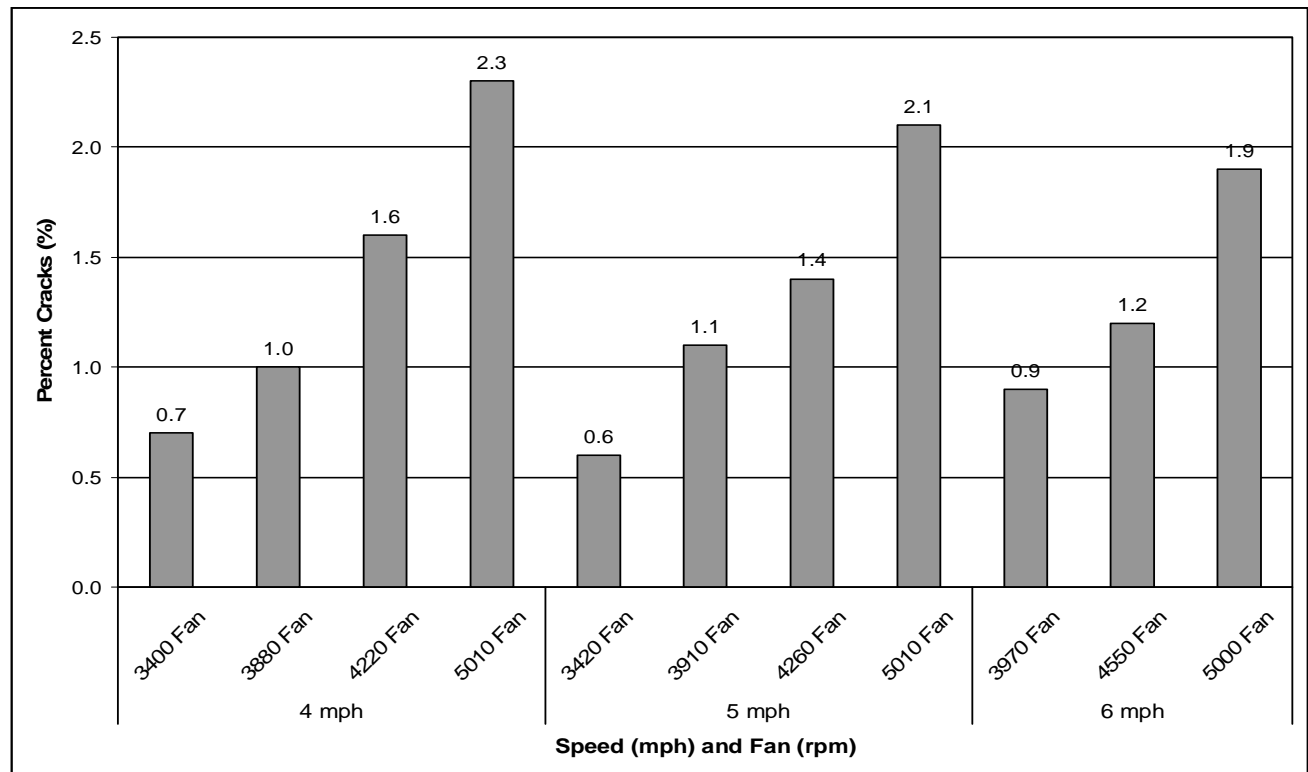
Figure 1. Effect of the Flexi-Coil Ground and Fan Speeds on Chickpea Damage.
