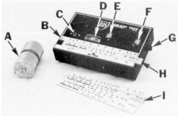
FIGURE 1. RDS Grain Test 2 Moisture Meter: (A) Test Cell, (B) Meter Scale, (C) Power Switch, (D) Meter Indicator, (E) Meter Reading, (F) Temperature Reading, (G) Build-in Temperature Sensor, (H) Sliding Crop Scale, (I) Additional Crop Scales.
