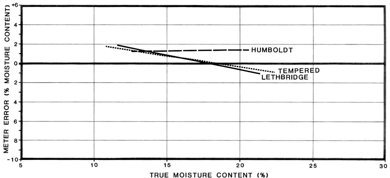
Figure 6. Deviations of Meter Readings for Skuttle MT2 in Three Different Types of Spring Wheat.
