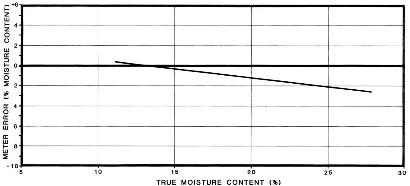
Figure 4. Deviations of Meter Readings for the Debnhorst G-6B in Oats.
