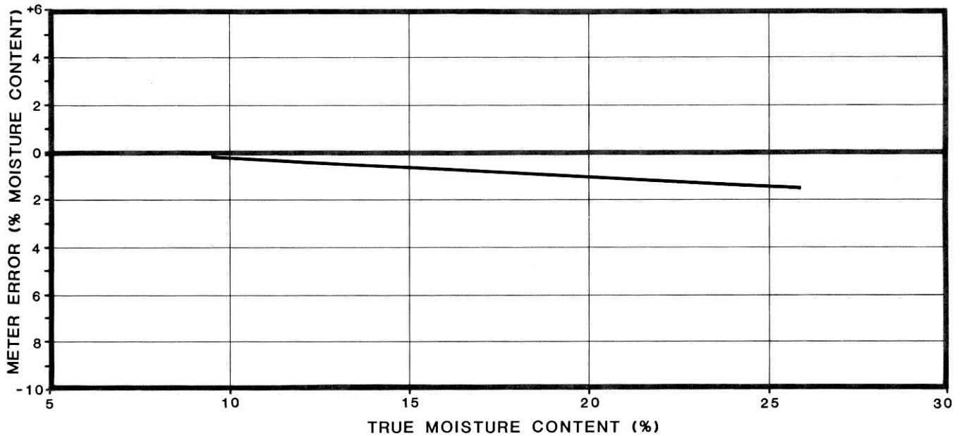
Figure 2. Deviations of Meter Readings for the Delmhorst G-6B in Wheat.
