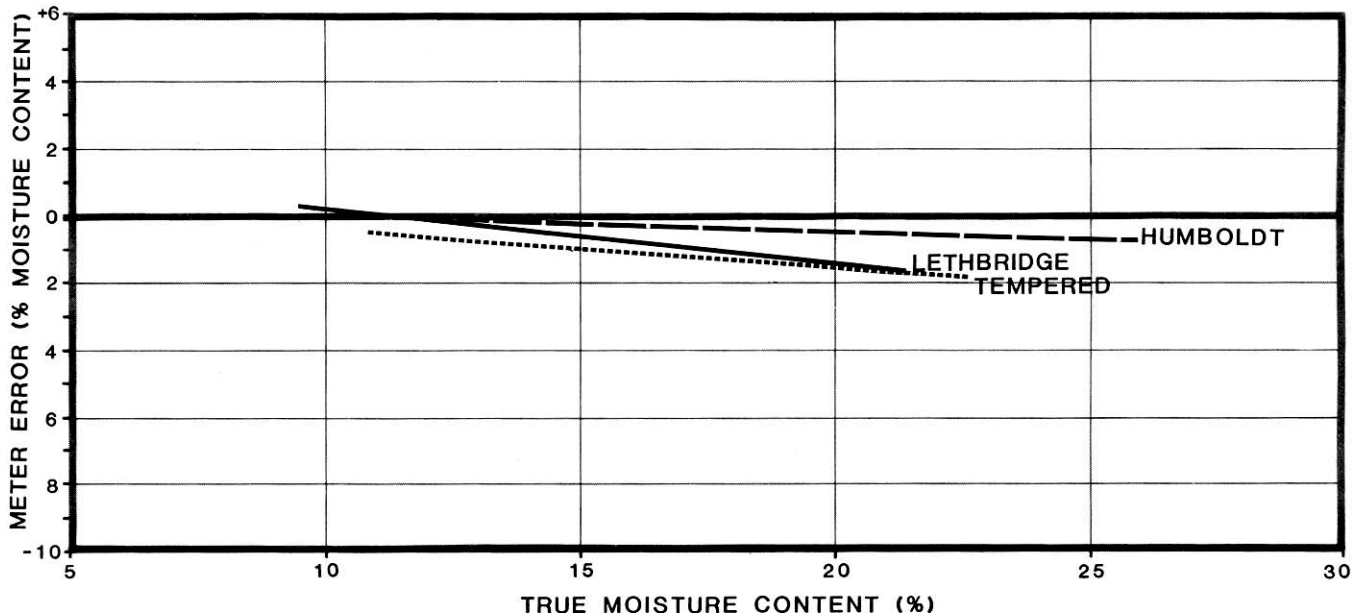
Figure 6. Deviations of Meter Readings for Delmhorst G-6B in Three Different Types of Spring Wheat.
