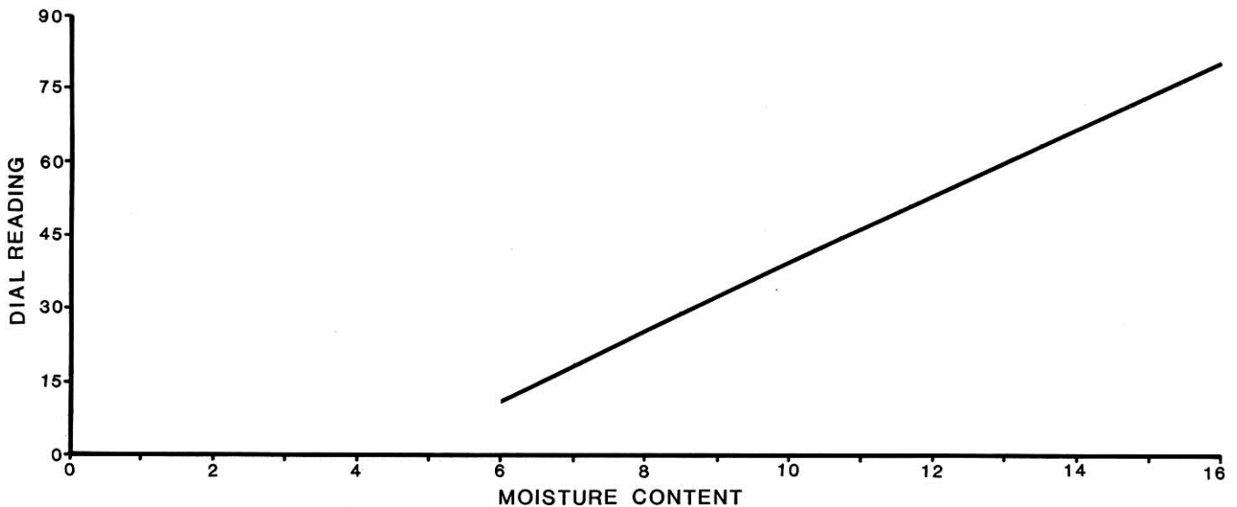
Figure 5. Calibration Curve for the Delrnhorst G-6B in Rapeseed.
