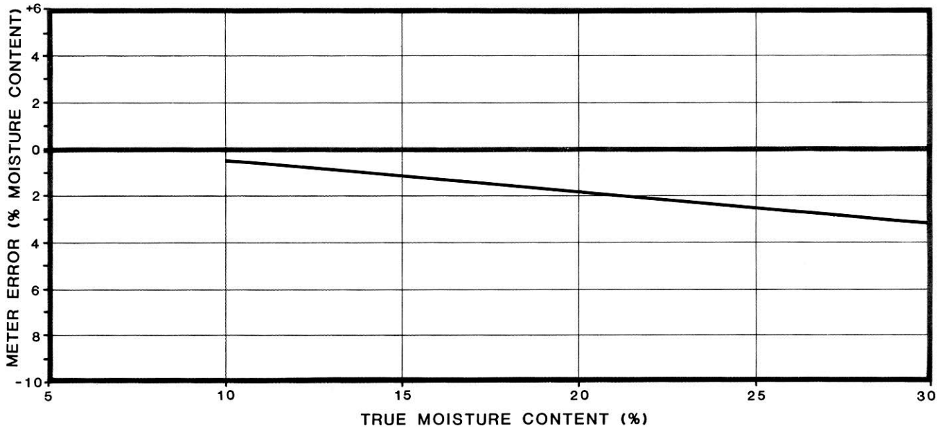
Figure 3. Deviations of Meter Readings for the Delmhorst G-6B in Barley.
