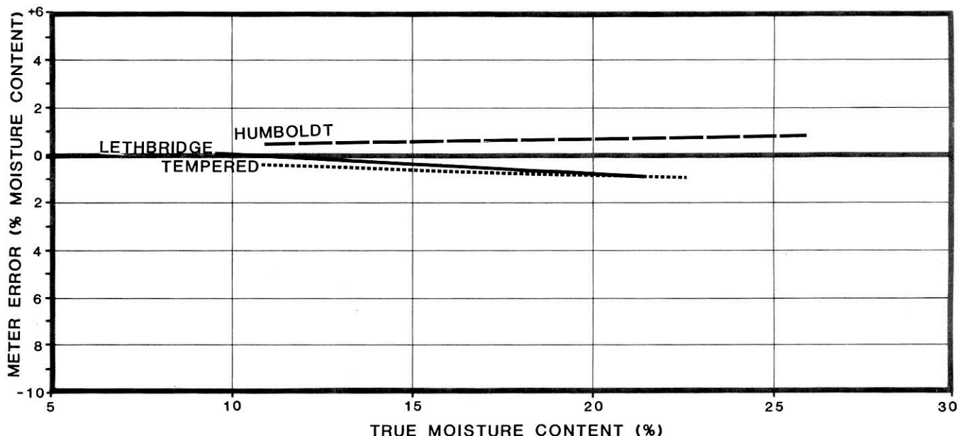
Figure 6. Deviation of Meter Readings for Dole 400 in Three Different Types of Spring Wheat.
