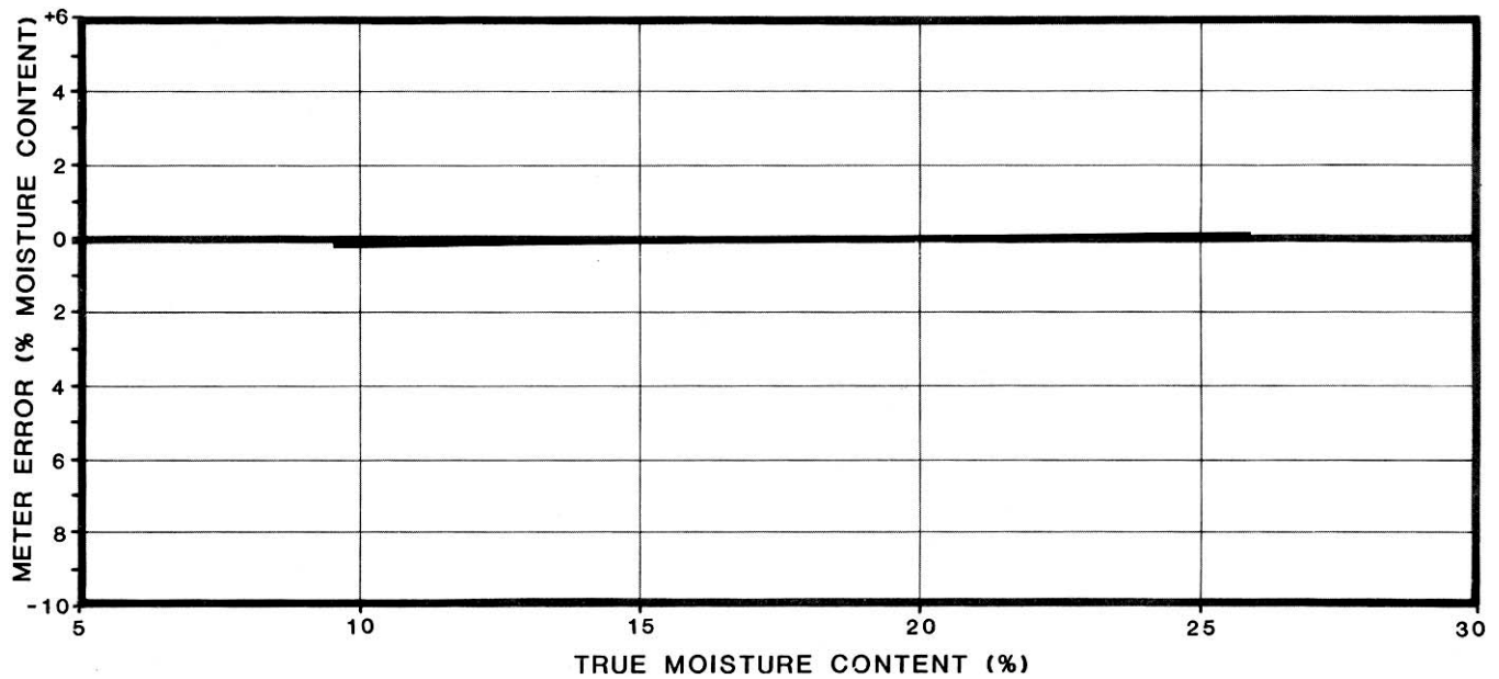
Figure 2. Deviations of Meter Readings for Dole 400 in Wheat.
