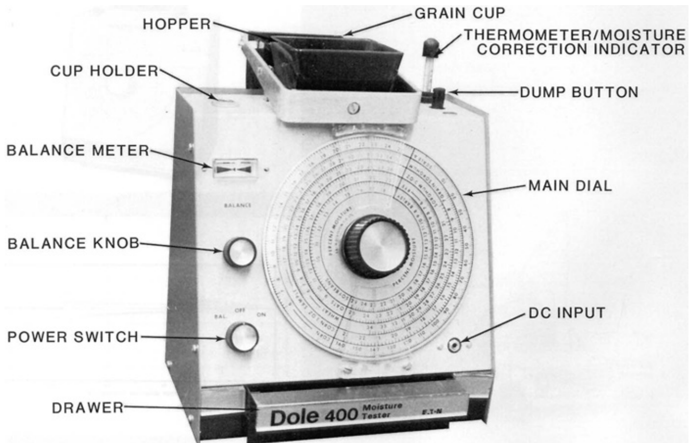
Figure 1. Detailed View of Dole 400 Grain Moisture Tester.
