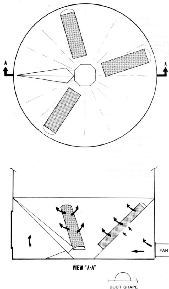
FIGURE 7. Westeel Coot Natural Air Drying System
