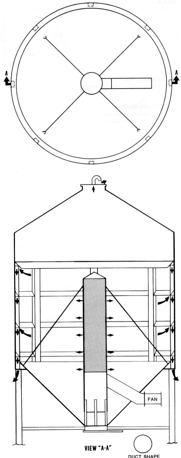
FIGURE 6. Univision Ultra-Dry Natural Air Drying System.
