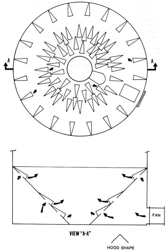
FIGURE 3. Harvest Hopper Natural Air Drying System.
