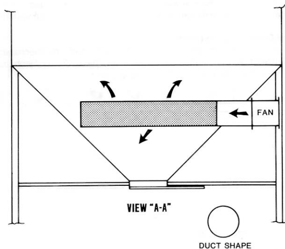
FIGURE 5. Univision In-Line Natural Air Drying System.
