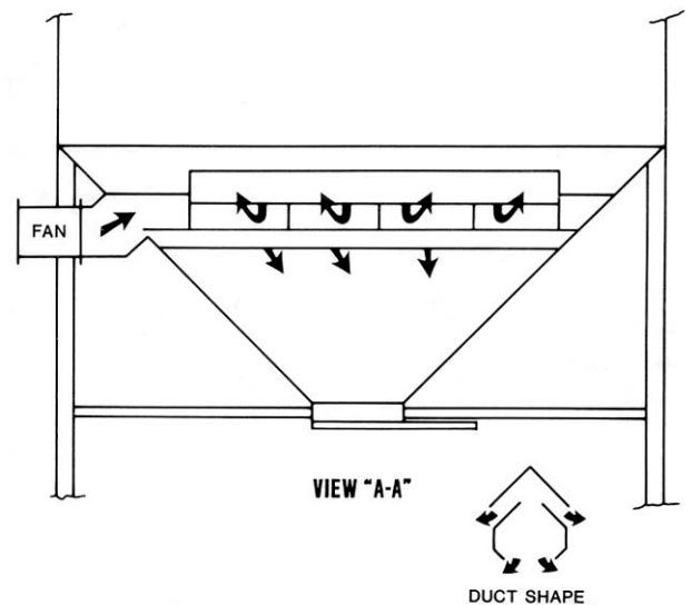
FIGURE 4. Trail Rite V Aeration Natural Air Drying System
