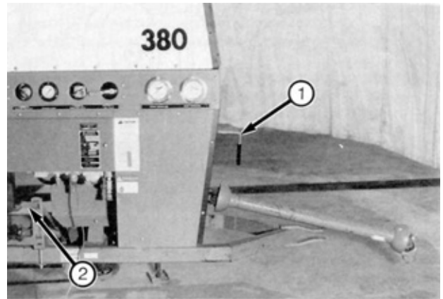
FIGURE 4. Controls: (1) Fan Clutch Lever, (2) Loading Auger Clutch Lever.
