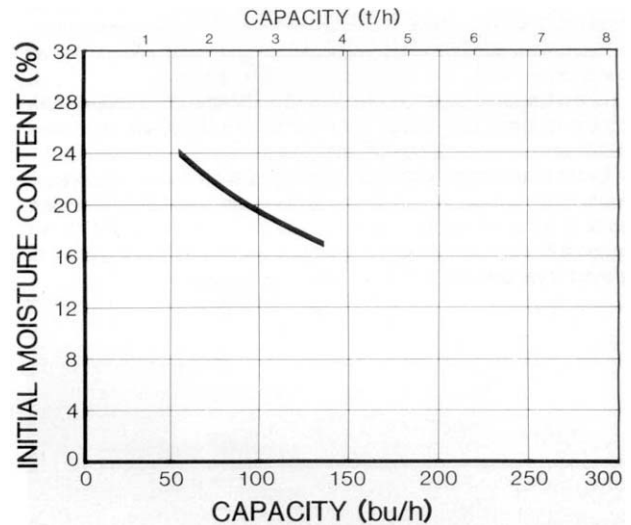
FIGURE 11. Drying Capacity in Wheat.
