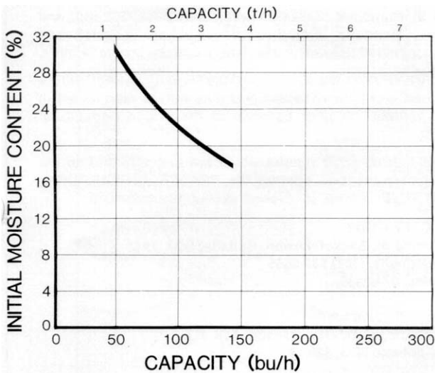
FIGURE 14. Drying Capacity in Corn (Hybrid 3996).
