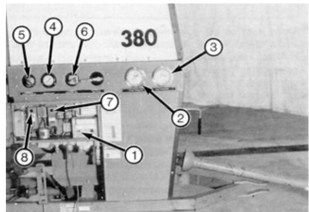
FIGURE 5. Controls and Instruments: (1) Power Switch, (2) Drying Air Temperature Gauge, (3) Grain Temperature Gauge, (4) Fuel Pressure Gauge, (5) Pressure Regulator Valve, (6) Modulating Valve, (7) Grain Temperature Control, (8) High Limit Switch.
