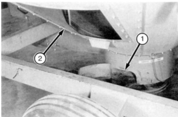
FIGURE 10. Access Doors. (1) Cleanout Door, (2) Dryer Access Door.
