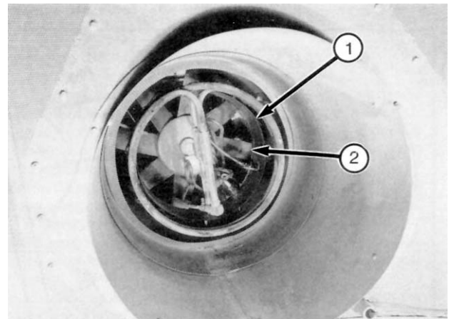
FIGURE 3. Fan Housing: (1) Burner, (2) Fan.
