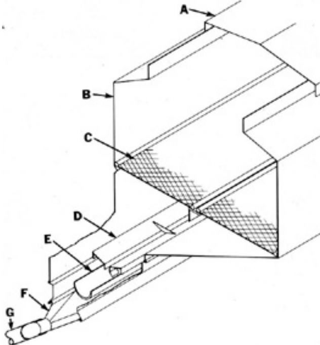
FIGURE 1. Spierco M80: (A) Lid, (B) Box, (C) Diamond Mesh Screen, (D) Baffle, (E) Oscillator, (F) Spout, (G) Delivery Tube.
