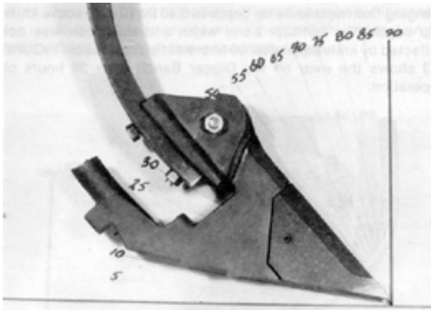
FIGURE 6. Culti-Band QC15 Knife Mounted on a Cultivator Shank.
