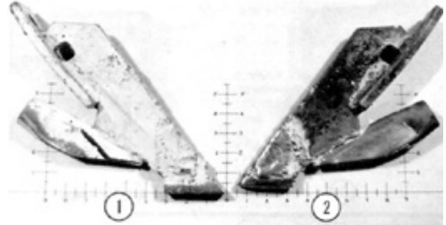
FIGURE 16. JAD Opener: 1) New, 2) Used.
