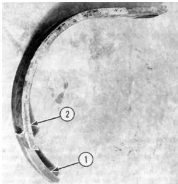
FIGURE 11. Shank Comparison: 1) Regular, 2) Cut-off and Modified.
