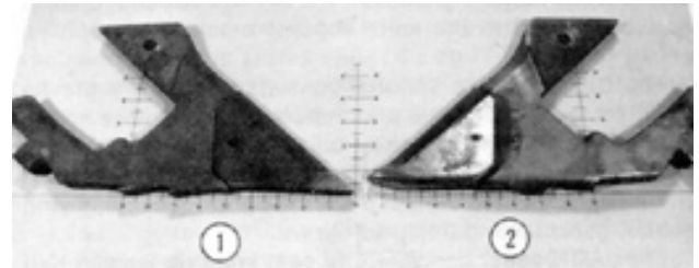
FIGURE. Culti-Band QC115: 1) New, 2) Used.
