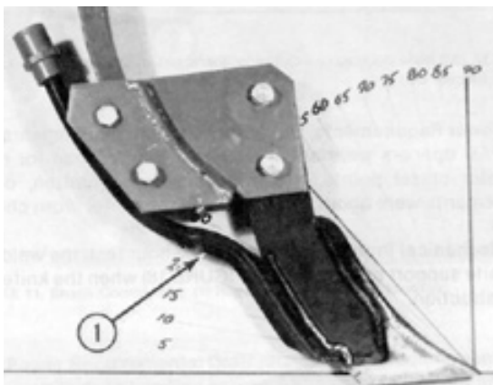
FIGURE 20. TSL Knife Mounted on a Cultivator Shank: 1) Location of Fertilizer Plugging.
