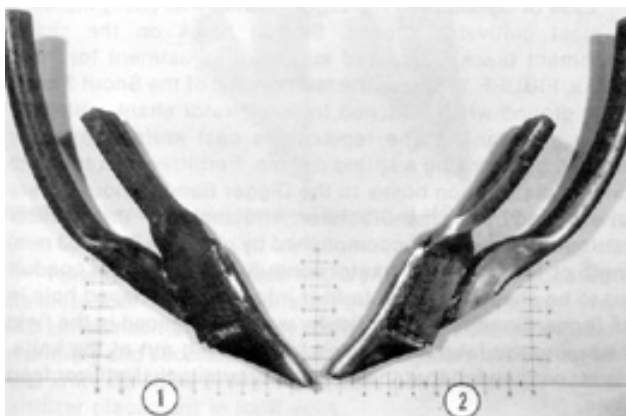
FIGURE 8. Dutch Granular Knife Number 7: 1) New, 2) Used.
