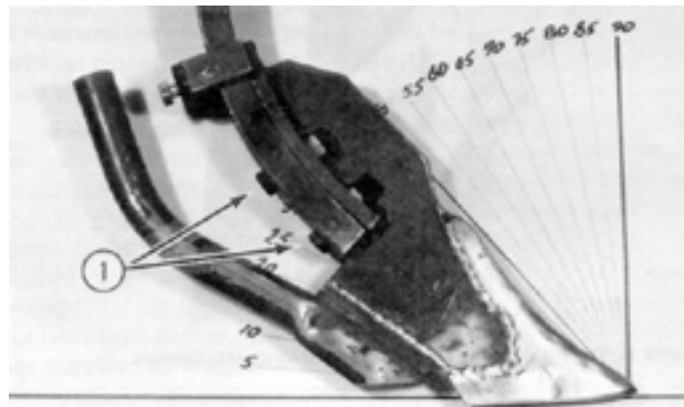
FIGURE 22. Haley Knife Mounted on a Cultivator Shank: (1) Limited Access to the Support Bracket Bolt Holes.
