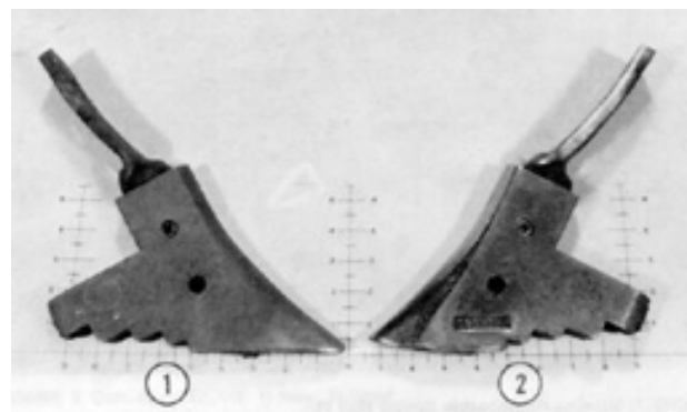
FIGURE 13. Digger Bandit Snout 3: 1) New, 2) Used.
