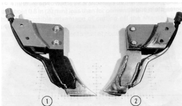
FIGURE 19. TSL Deep Banding Knife: 1) New, 2) Used.
