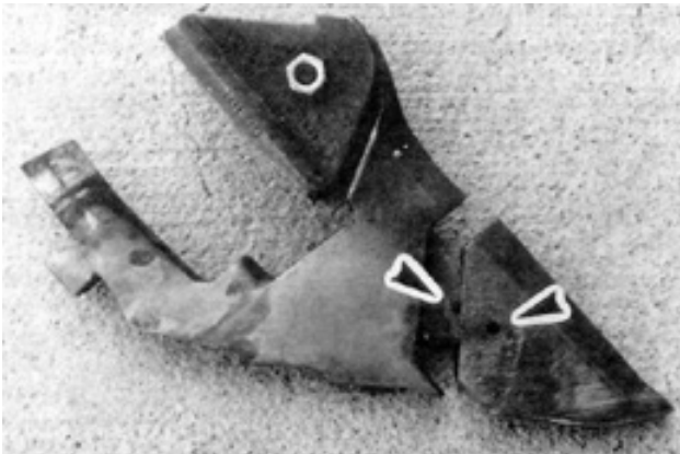
FIGURE 7. Missing Replaceable Spring Roll Pin.
