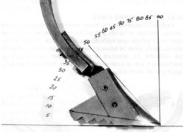
FIGURE 14. Digger Bandit Knife Mounted on a Cultivator Shank.
