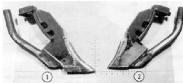
FIGURE 21. Haley Side Bander: 1) New, 2) Used.
