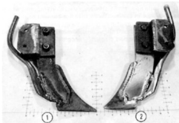
FIGURE 10. Gromor Deep Banding Knife: 1) New, 2) Used.
