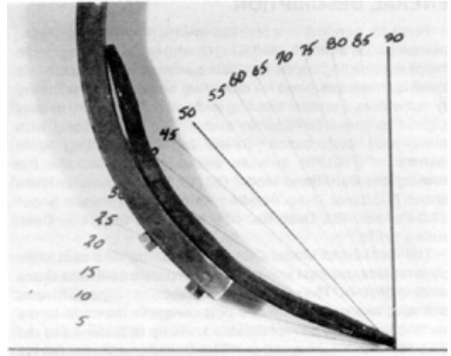
FIGURE 4. Conventional Cultivator Chisel Point Mounted on a Cultivator Shank.
