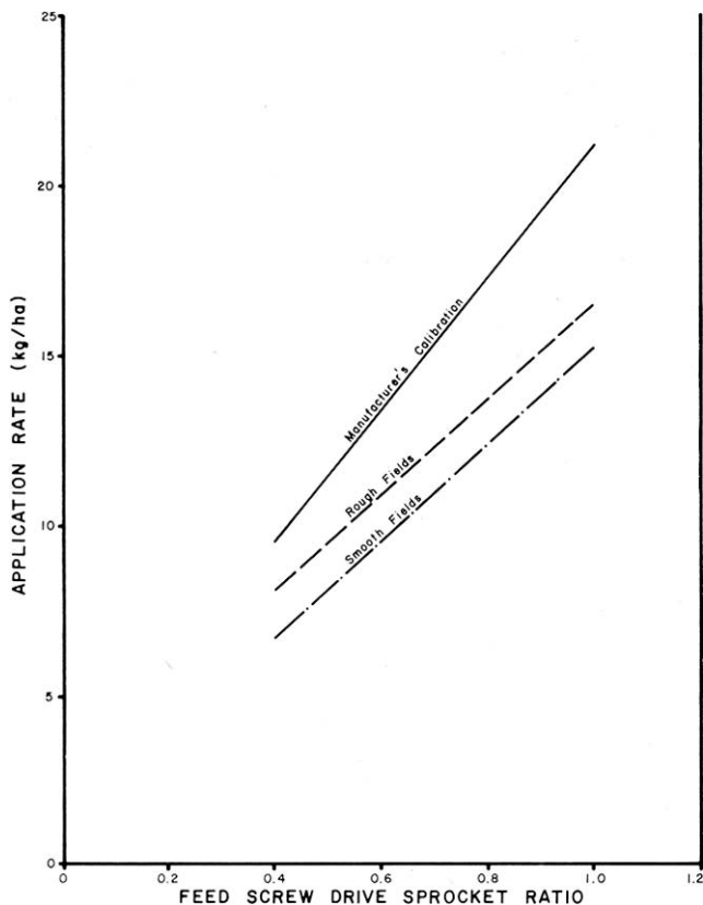
FIGURE 2. Calibration Curves for Avadex BW.
