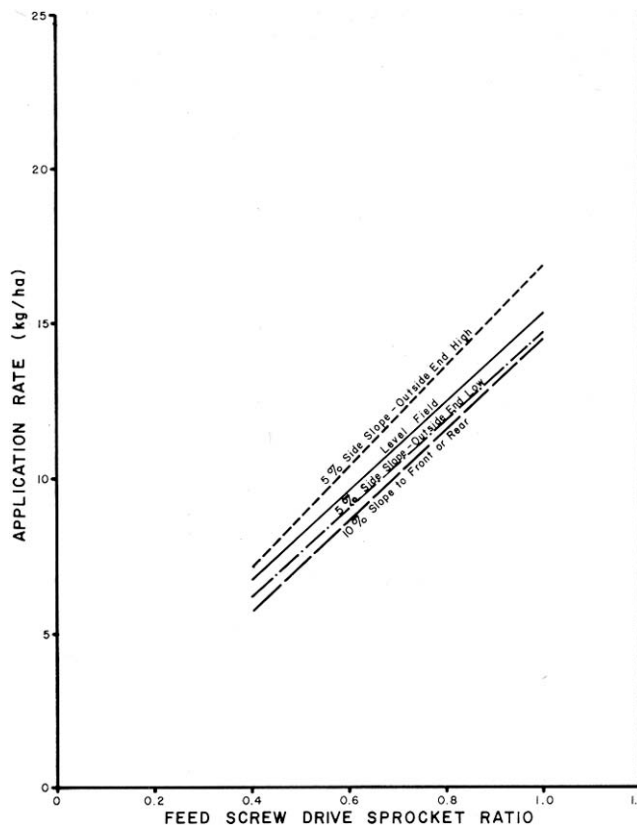
FIGURE 3. Effect of Field Slope on Application Rate of Avadex BW.
