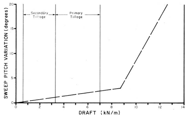
FIGURE 13. Sweep Pitch Variation over a Normal Range of Draft (305 mm Shank Spacing).
