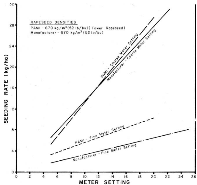
FIGURE 5. Metering Accuracy in Rapeseed.
