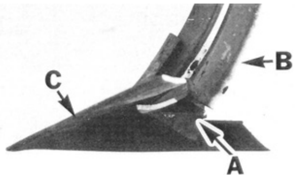
FIGURE 9. Friggstad Seed Boot: (A) V-shaped Deflector, (B) Seed Boot, (C) Sweep.
