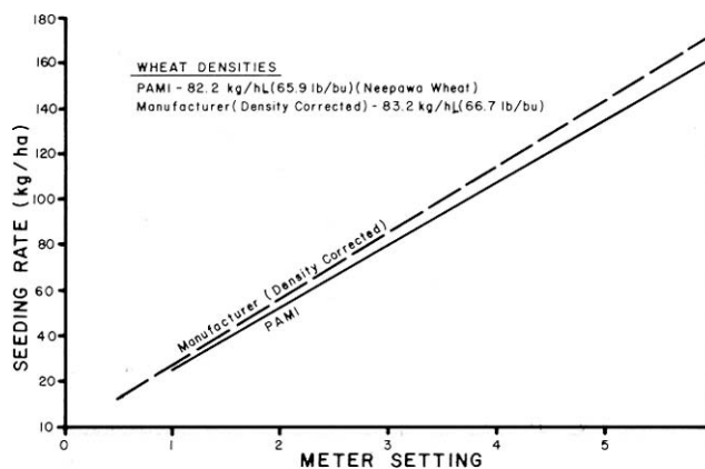
FIGURE 2. Metering Accuracy in Wheat.
