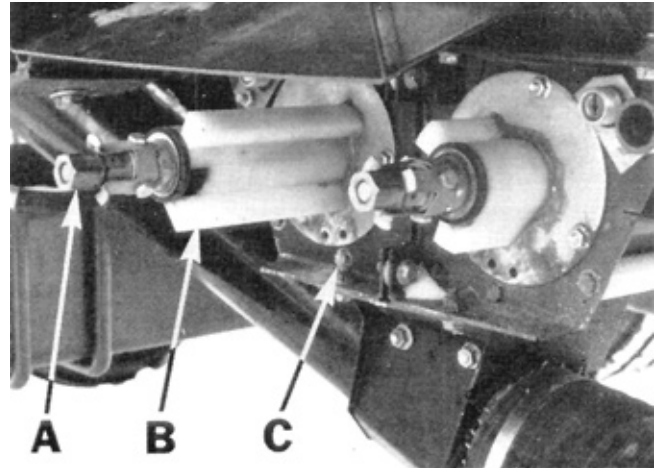
FIGURE 18. Application Rate Adjustment: (A) Threaded Adjusting Screw, (B) Exposed Flute, (C) Feed Gate Adjustment.
