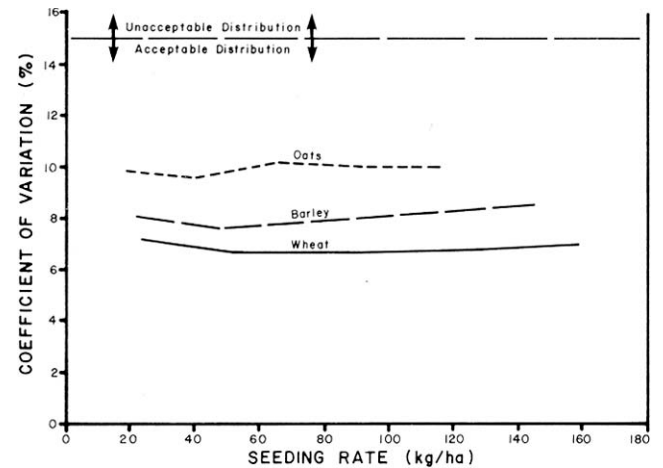
FIGURE 7. Seeding Uniformity in Cereal Grains at 9 km/h.
