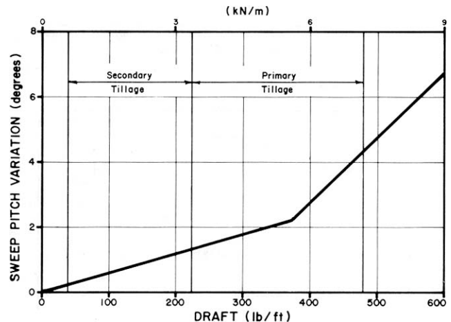
FIGURE 14. Sweep Pitch Variation Over a Normal Range of Draft with 12 in (305 mm) Shank Spacing.
