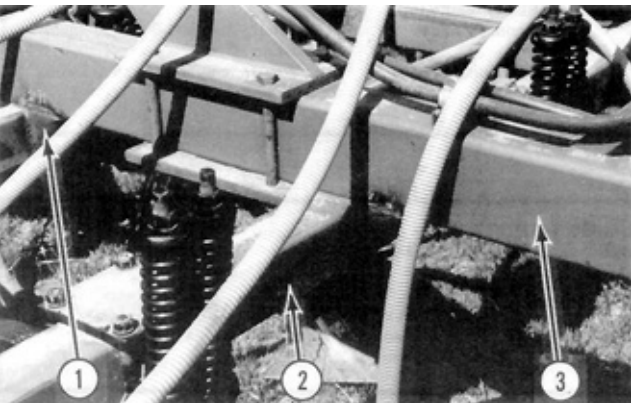
FIGURE 24. Cultivator Frame Reinforcing: (1) Gussets, (2) Lift Member, (3) Lateral Members.
