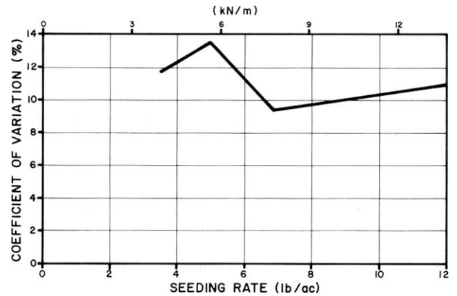
FIGURE 10. Distribution Uniformity in Canola Over a Range of Seeding Rates at 5.5 mph (9 km/h) at a Fan Speed of 4500 rpm.
