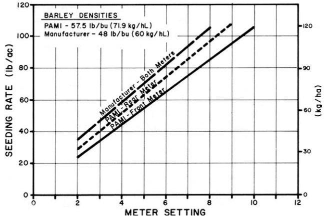
FIGURE 3. Metering Accuracy in Barley.
