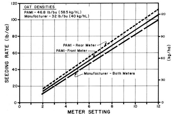
FIGURE 4. Metering Accuracy in Oats.
