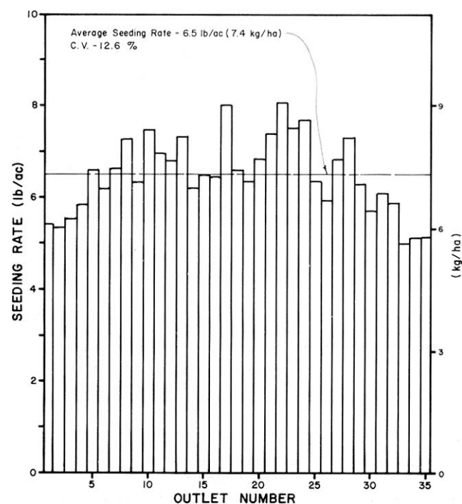
FIGURE 9. Distribution Uniformity Pattern in Canola at 6.5 lb/ac (7.4 kg/ha) at a Fan Speed of 2000 rpm.
