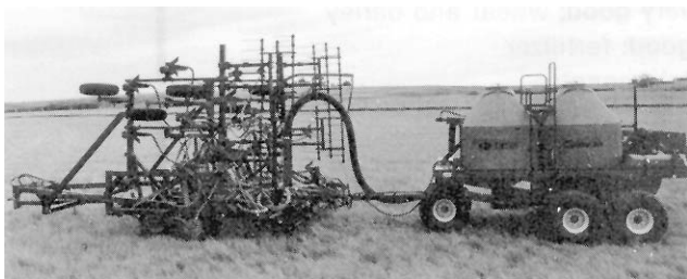
FIGURE 13. Transport Position.
