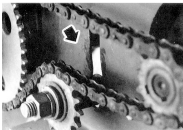
FIGURE 15. Idler Sprocket and Bent Frame.
