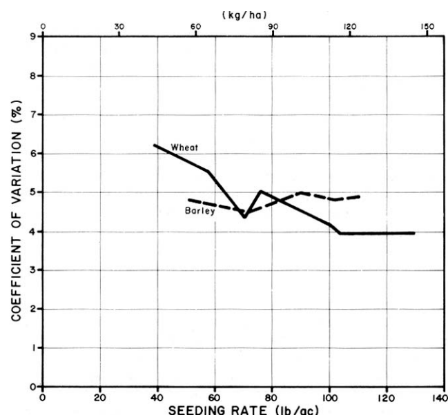
FIGURE 7. Distribution Uniformity in Cereal Grains over a Range of Seeding Rates at 5.0 mph (8 km/h) at Varying Fan Speeds.
