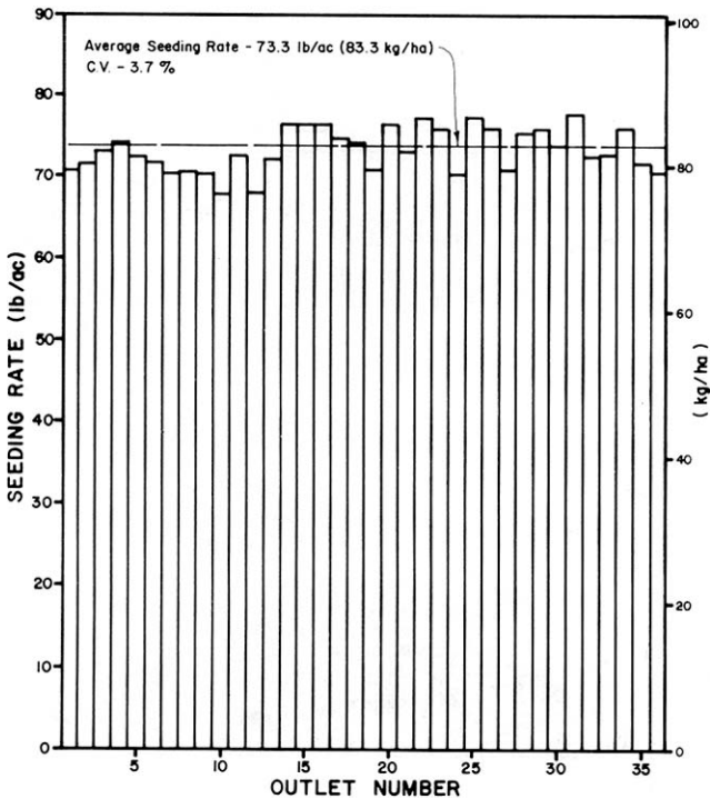
FIGURE 8. Distribution Uniformity Pattern in Wheat at 73.3 lb/ac (83.3 kg/ha) at a Fan Speed of 2320 rpm.
