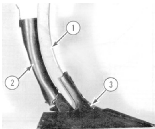
FIGURE 2. Flexi-coil 1600 Seed Boot: (1) Shank, (2), Seed Boot, (3) Sweep.
