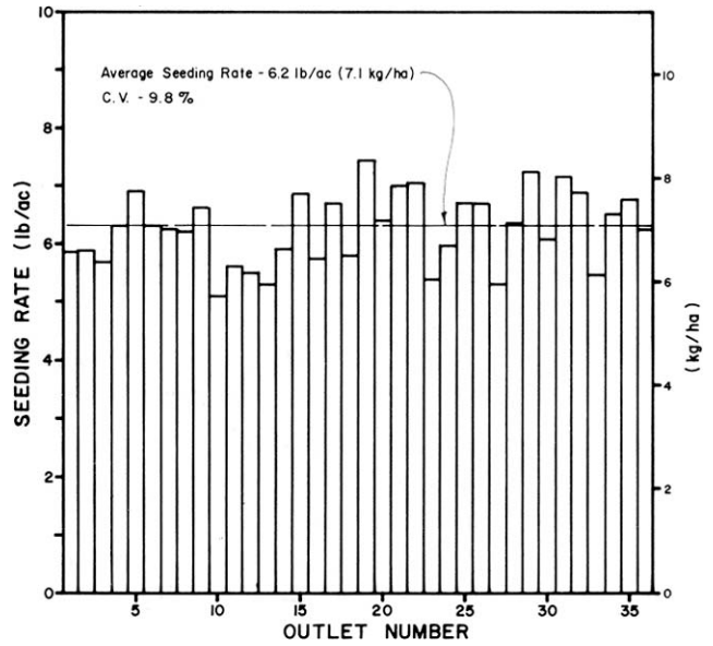
FIGURE 9. Distribution Uniformity Pattern in Canola at 6.3 lb/ac (7.2 kg/ha) at a Fan Speed of 2230 rpm.
