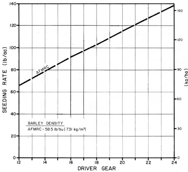
FIGURE 9. Metering Accuracy in Barley.
