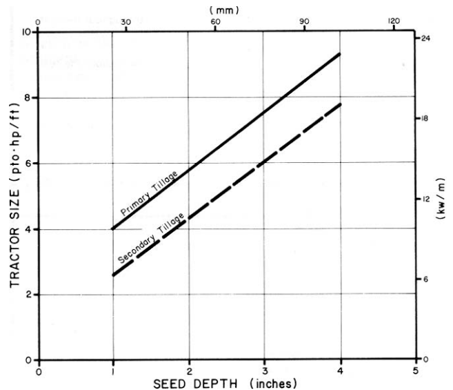
FIGURE 24. Average Horsepower Requirements at 5 mph (8 km/h).
