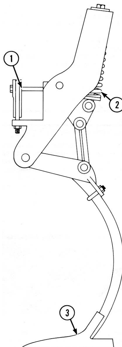
FIGURE 3. Shank Assembly: (1) Frame Mounts, (2) Trip Spring, (3) Sweep.
