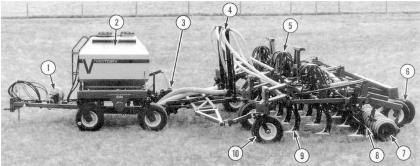
FIGURE 1. Victory Seed-o-Vator: (1) Centrifugal Fan, (2) Tanks, (3) Ground Engaging Meter Drive Wheel, (4) Primary Header, (5) Secondary Header, (6) Transport Wheels, (7) Steel Press Wheels, (8) Rod Weeder, (9) Shank Opener, (10) Cultivator Castor Gauge Wheel.
