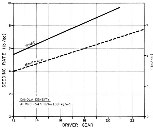
FIGURE 10. Metering Accuracy in Canola.
