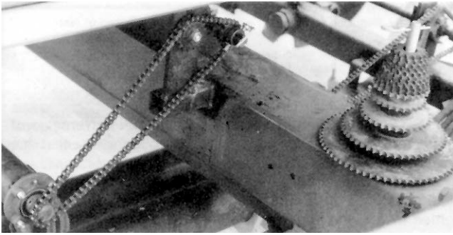
FIGURE 21. Metering Sprockets.
