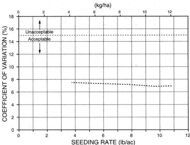
FIGURE 14. Distribution uniformity with canola over a range of seeding rates.
