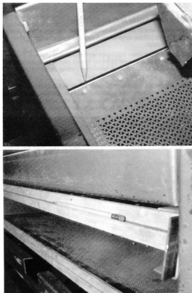
FIGURE 4. Screen Frame Positioning and Separation.
