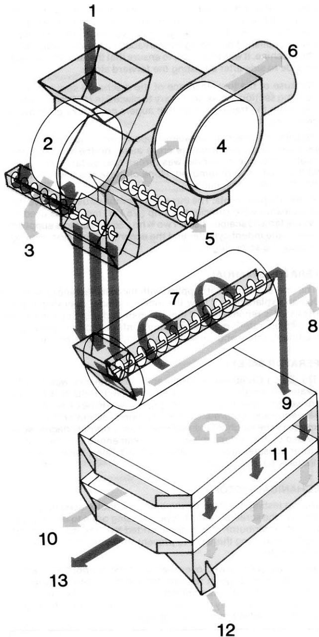
FIGURE 3. Material Flow Diagram: (1) Inlet Hopper, (2) Scalper Disks, (3) Large Coarse Material, (4) Fan, (5) Light Material, (6) Chaff, (7) Indent Cylinder, (8) Long Material, (9) Large Screen, (10) Coarse Material, (11) Small Screen, (12) Fine Material, (13) Clean Grain.
