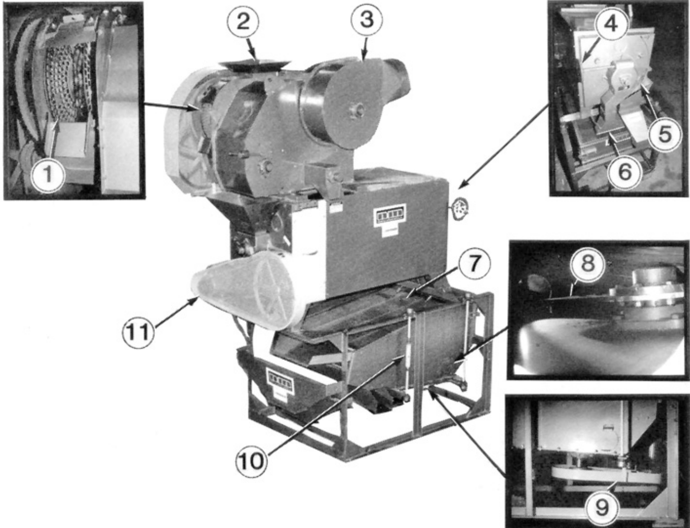
FIGURE 1. Bisco Cleaner: (1) Scalper Disks, (2) Inlet Hopper, (3) Centrifugal Fan, (4) Indent Cylinder Trough Adjustment, (5) Indent Cylinder Retarder, (6) Grain Distributor, (7) Screens, (8) Counter Balance Weight, (9) Eccentric Drive System, (10) Screen Slope Adjustment, (11) Indent Cylinder Drive System.
