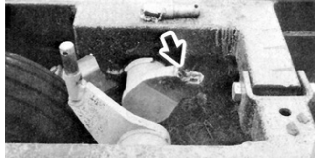
FIGURE 10. Turnbuckle Pin Failure.
