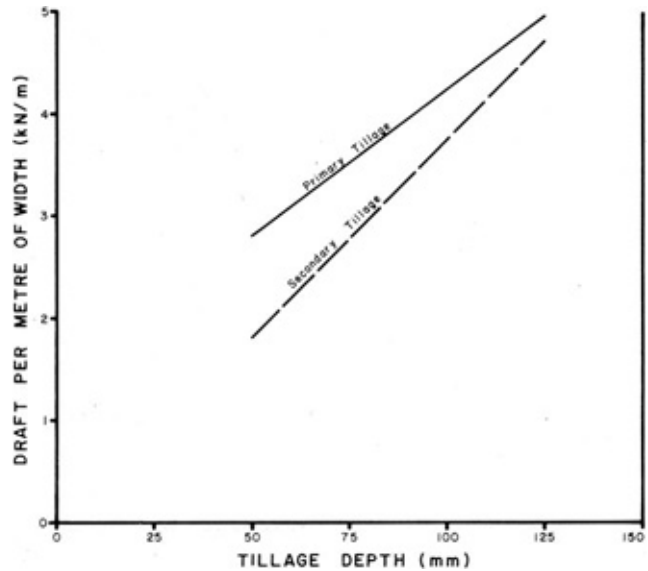
FIGURE 9. Average Draft Requirements for Blade Cultivators at 8 km/h.
