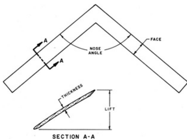
FIGURE 2. Blade Terminology.
