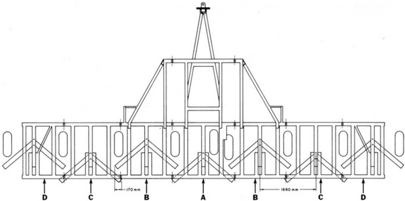
FIGURE 4. Blade Pattern Showing Wheel Location, Shank Spacing and Blade Overlap: (A) Centre Section, (B) Centre Wing Sections, (C) Extension Wing Sections, (D) Outer Wing Sections.
