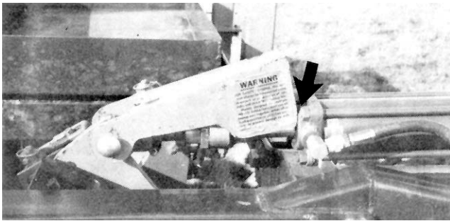
FIGURE 8. Interference Between Transport Locks and Depth Control Stop Collars.
