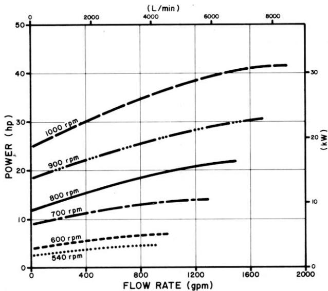
FIGURE 3. Power Requirements to Operate the Lloyd's Model RE-80 Pump at Various Flow Rates and Power Take-off Speeds.
