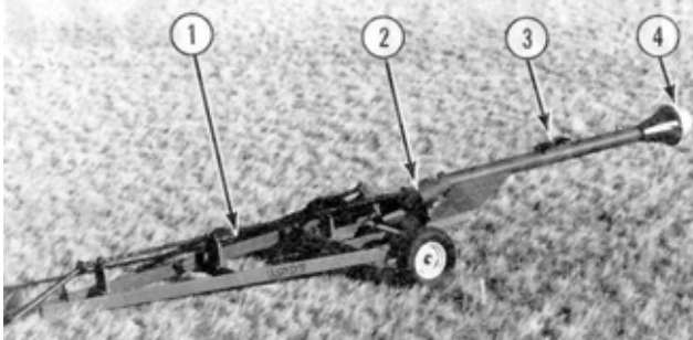
FIGURE 1. Lloyd's Model RE-80 Lift Pump: (1) Lift Mechanism, (2) Discharge Tube, (3) Bearing Inspection Plate, (4) Impeller.
