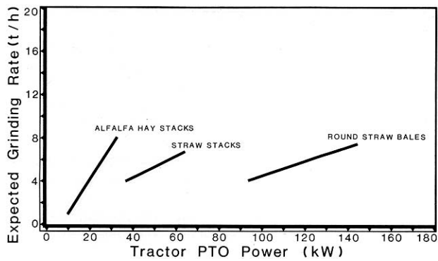
FIGURE 7. Determining Expected Average Grinding Rates With the New Holland 379 for Various Tractor Sizes when Using a 51 mm (2 in) Screen.
