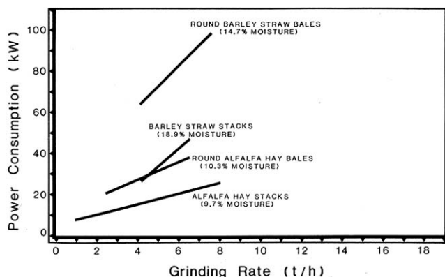
FIGURE 5. Power Consumption of the New Holland 379 at Various Grinding Rates, when Equipped with a 51 mm (2 in) Screen.
