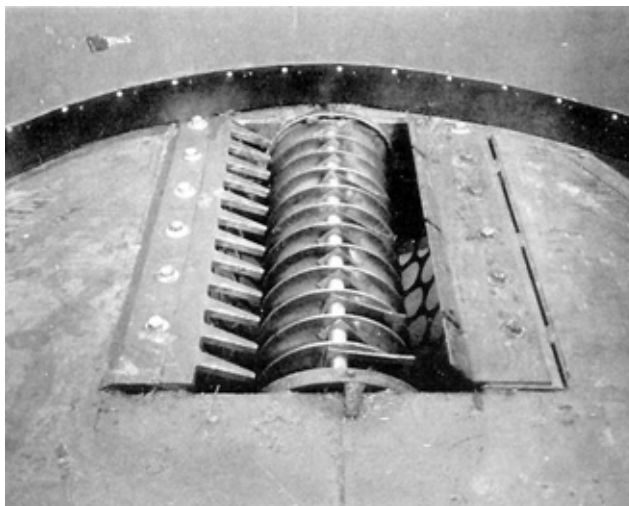
FIGURE 3. Hammer Mill and Screen.
