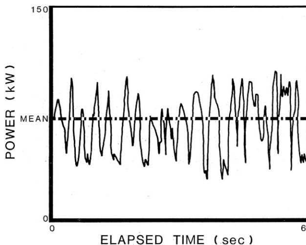
FIGURE 6. Typical Instantaneous Power Requirements for a Tub Grinder.
