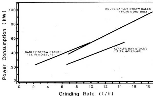
FIGURE 5. Power Consumption of the Haybuster H-1000, at Various Grinding Rates, when Equipped with a 51 mm (2 in) Screen.
