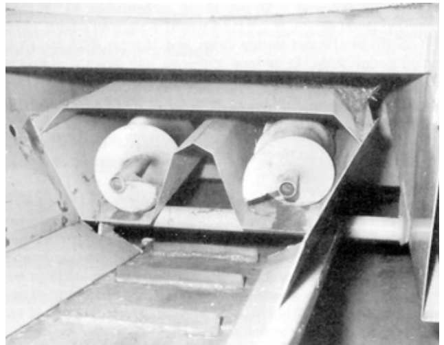
FIGURE 4. Belly Pan Auger.
