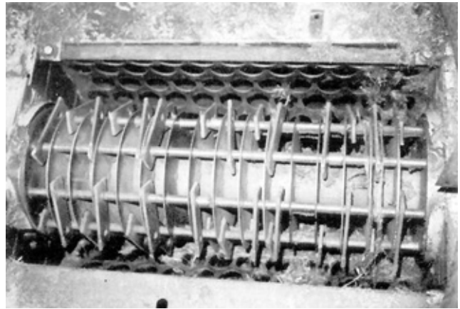
FIGURE 3. Hammer Mill and Screen.
