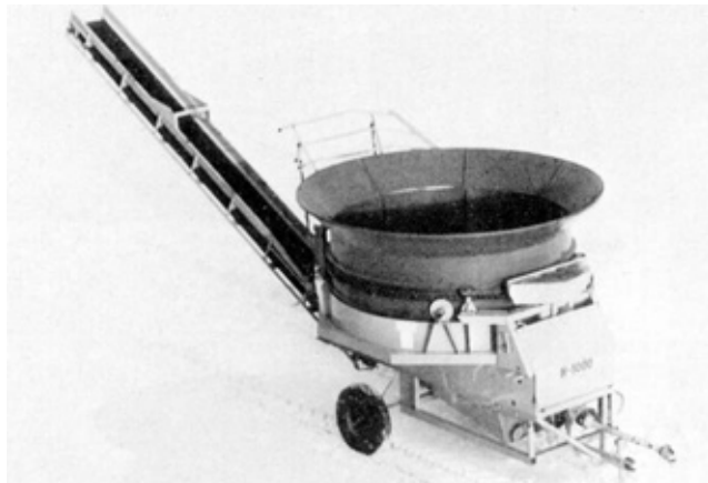
FIGURE 1. Haybuster H-1000 Tub Grinder.
