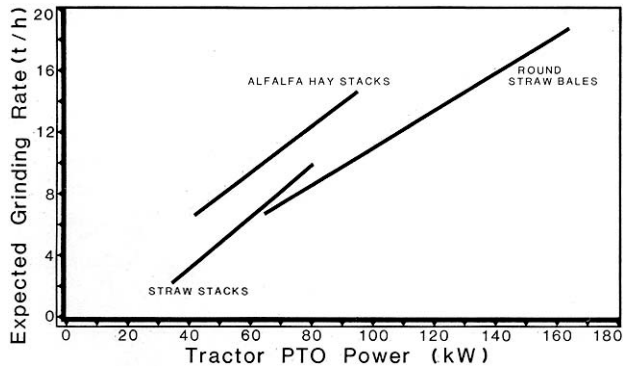
FIGURE 7. Determining Expected Average Grinding Rates with the Haybuster H-1000 for Various Tractor Sizes when Using a 51 mm (2 in) Screen.
