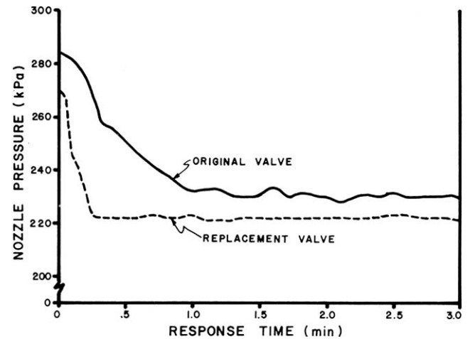
FIGURE 8. Response Time for Two Motorized Control Valves to Changes in Forward Speed.
