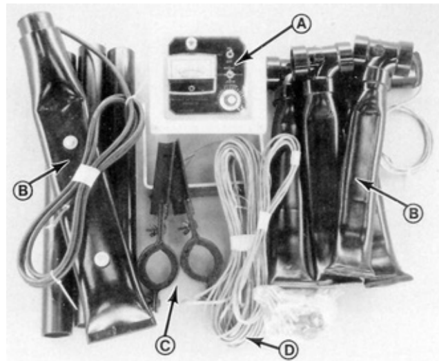
FIGURE 1. Sens-Saver SS2 Grain Loss Monitor: (A) Control Box (B) Sensor Assembly (C) Mounting Hardware (D) Wiring Harness.
