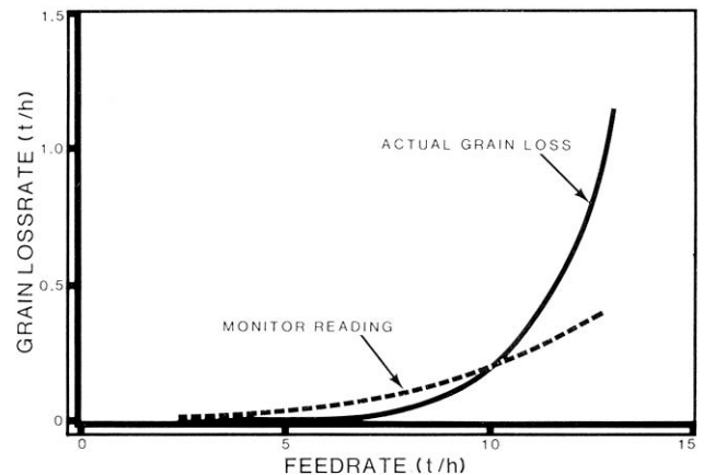
FIGURE 4. Comparison of Monitor Reading to Actual Combine Lossrate in a Field of Neepawa Wheat.
