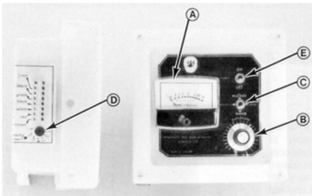
FIGURE 3. Control Box: (A) Loss Meter (B) Calibration Control (C) Sensor Selector Switch (D) Sensitivity Control (E) Power Switch.
