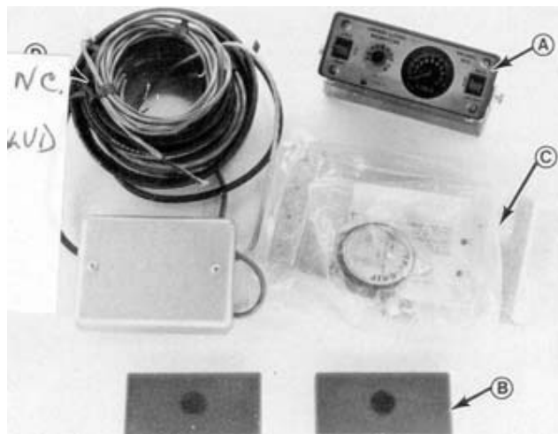
FIGURE 1. SED Model 912 Grain Loss Monitor: (A) Control Box (B) Sensors (C) Mounting Hardware (D) Wiring Harness
