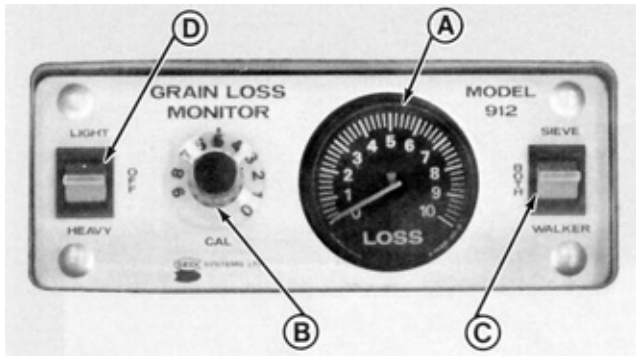
FIGURE 3. Control Box: (A) Loss Meter, (B) Calibration Control, (C) Sensor Selector, (D) Sensitivity Control and Power Switch.
