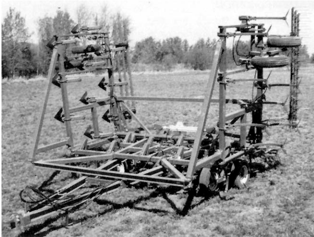
FIGURE 9. Transport Position.
