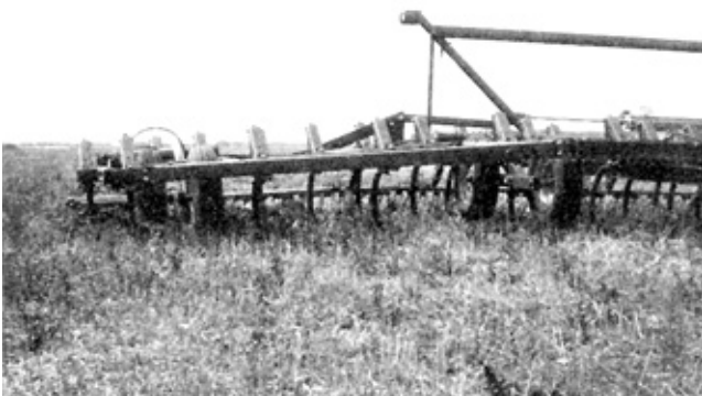
FIGURE 5. Excessive Wing End Penetration in Heavy Primary Tillage.
