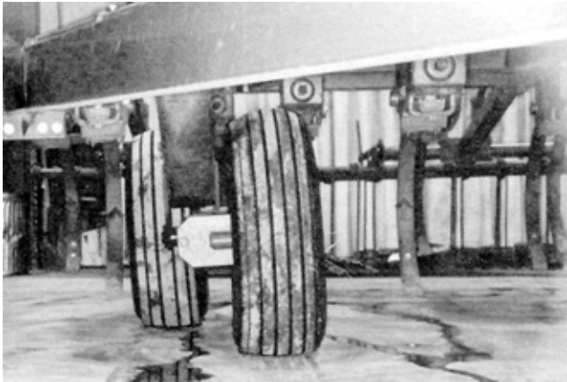
FIGURE 11. Centre Section Wheel Support Deflection in Transport Position.
