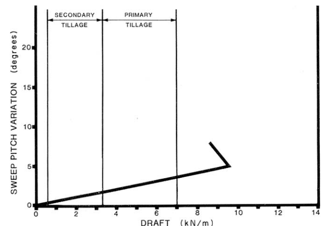
FIGURE 3. Sweep Pitch Variation Over a Normal Draft Range.
