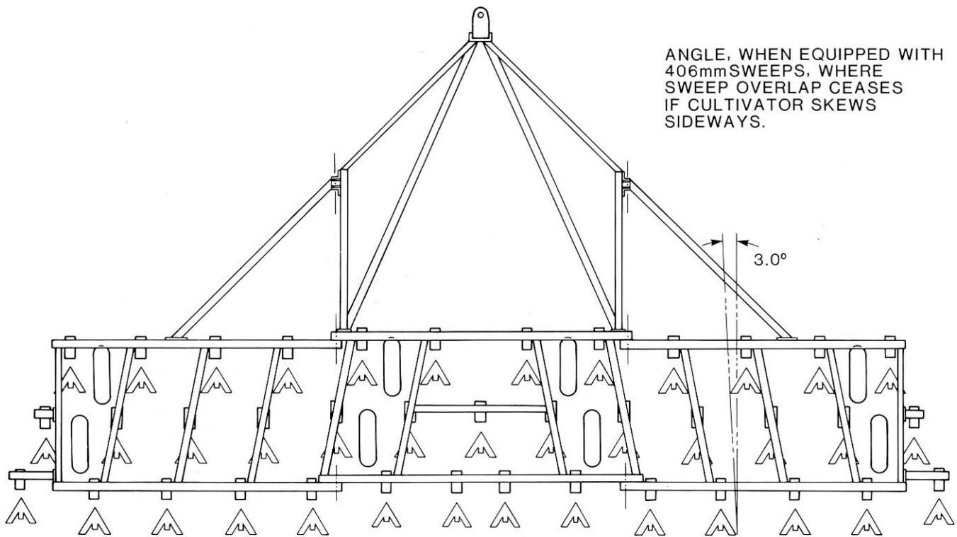
FIGURE 8. Sweep Pattern (305 mm Shank Spacing).
