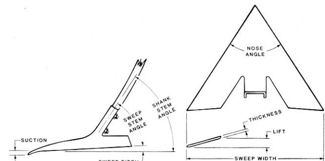
FIGURE 2. Shank and Sweep Terminology.
