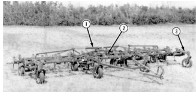
FIGURE 1. Flexi-coil 800: (1) Wing Lift Cylinders, (2) Depth Control Cylinder, (3) Outrigger Wheels.
