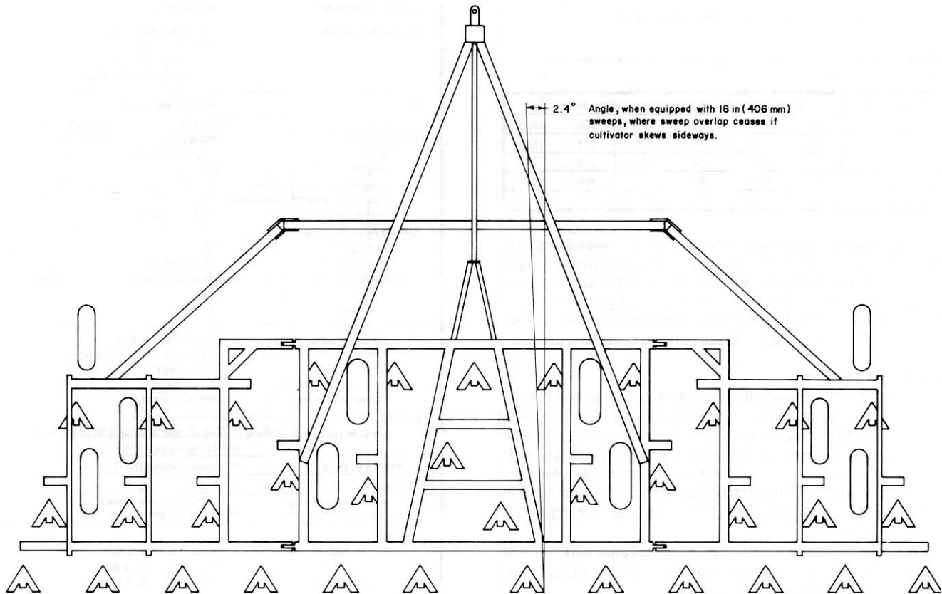
FIGURE 5. Sweep Pattern.
