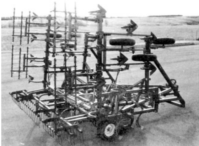
FIGURE 6. Transport Position.
