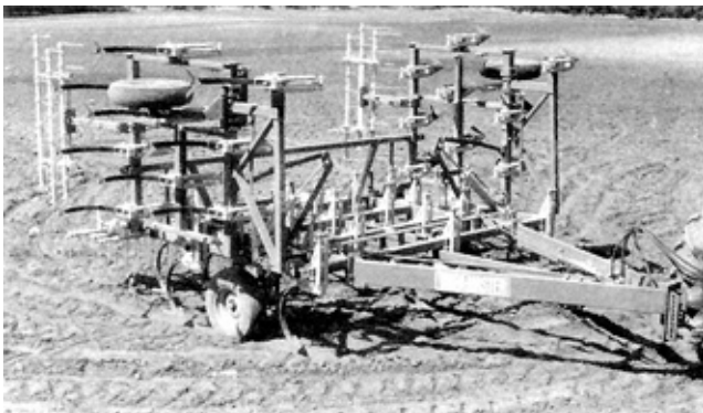
FIGURE 8. Transport Position.
