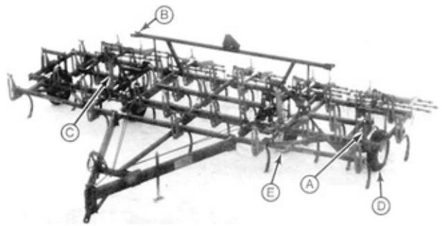
FIGURE 1. Bourgault Vibra-Master: (A) Depth Control Cylinder, (B) Wing Safety Stops, (C) Wing Lift Cylinder, (D) Wing Wheels, (E) Centre Wheels.
