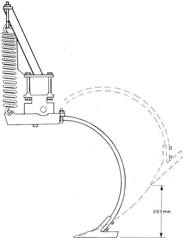
FIGURE 4. Shank Lifting Pattern.
