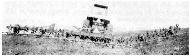
FIGURE 6. Ample Wing Flexibility when Pivoting Upward in Relation to Centre Frame.
