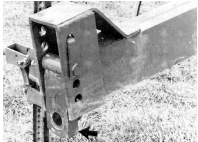
FIGURE 11. Hitch Link in Vertical Position.
