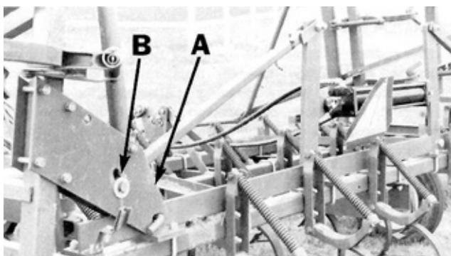
FIGURE 10. Wing Lift Linkage: (A) Wing Lift Bracket, (B) Slot.
