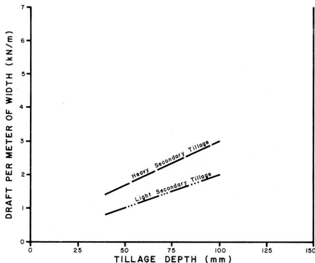
FIGURE 13. Average Draft Requirements for Field Cultivators at 8 km/h.
