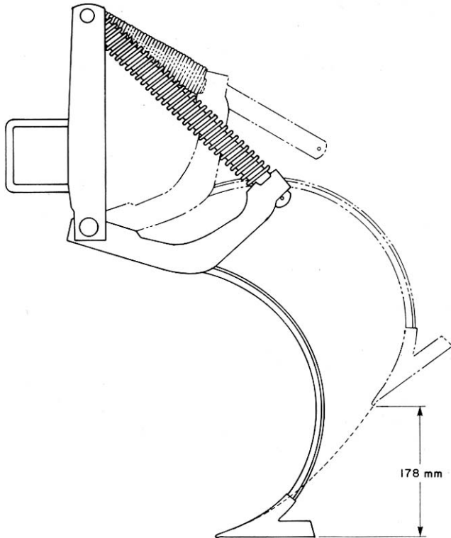
FIGURE 4. Shank Lifting Pattern (Spring Holder Tube in Normal Position).
