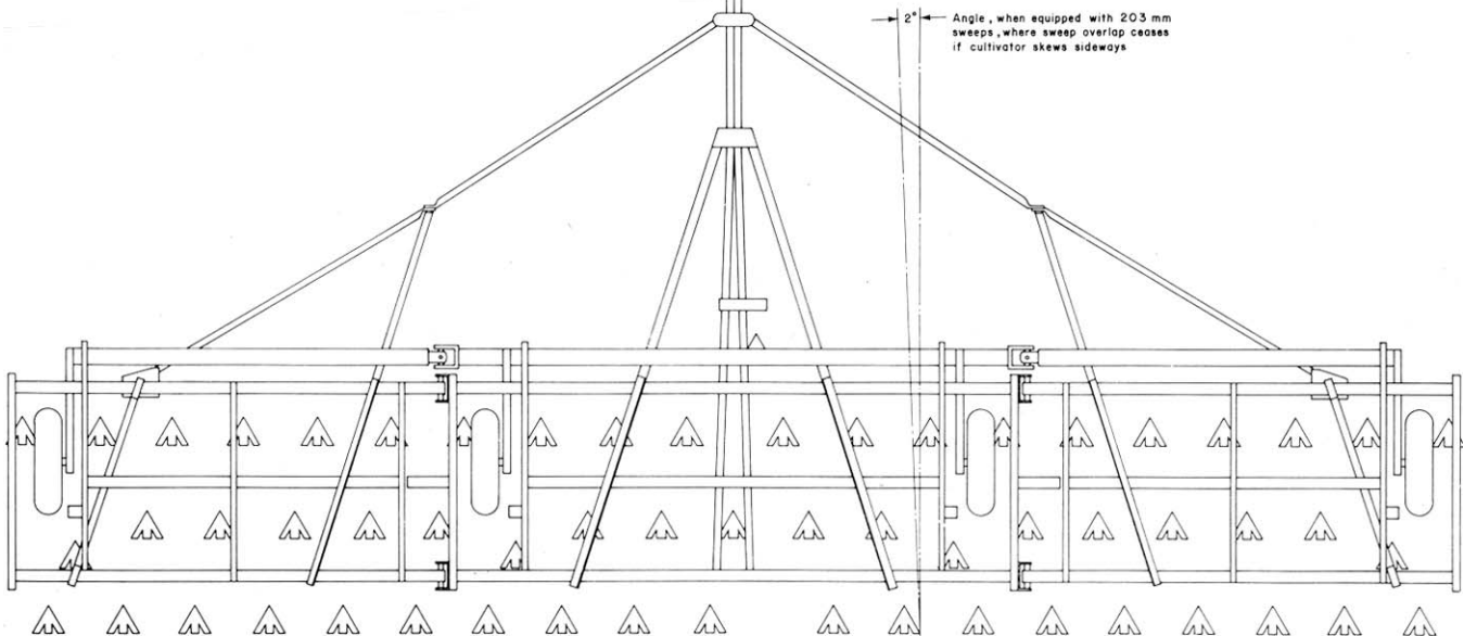
FIGURE 8. Sweep Pattern (165 mm shank spacing).
