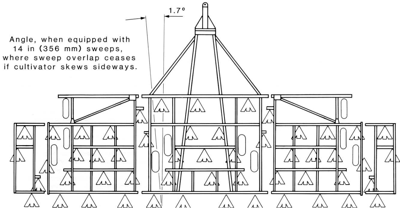
FIGURE 8. Sweep Pattern.
