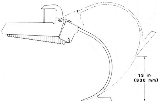
FIGURE 5. Shank Mechanism.
