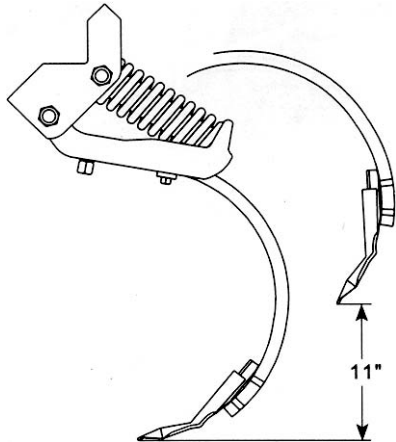
Figure 4. Flexi-coil 500 lb Shank Trip Mechanism.
