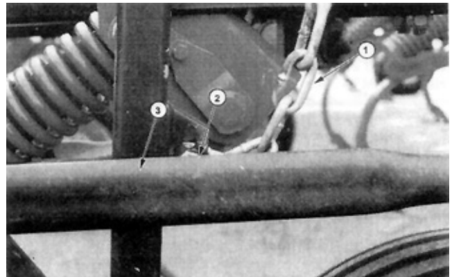
Figure 9. Restraint Chain Link Assembly: (1) Chain Link, (2) Lower Bolt and (3) Depth Link Adjustor Rod.
