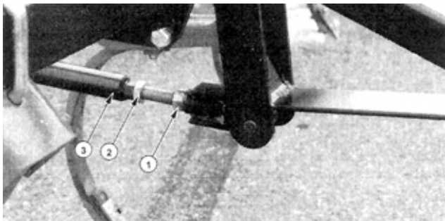
Figure 8. Depth Link Adjustor Assembly. (1) Adjusting Nut, (2) Jam Nut and (3) Depth Link Adjustor Rod.
